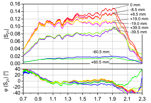
Figure 6: Results of Model Measurements
