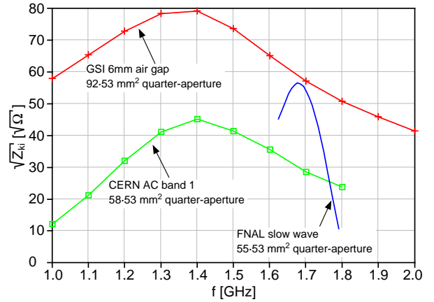
Figure 3: Comparison between different longitudinal kicker electrodes for \beta = 0.97 and a vertical distance of 53 mm to the beam
