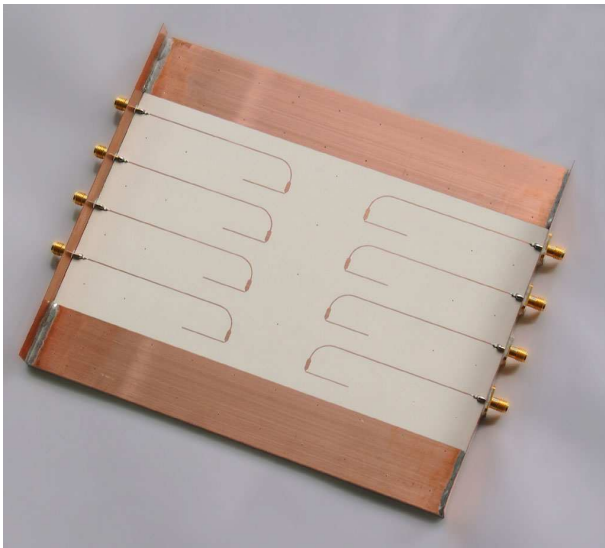
Figure 5: Slotline Electrode Model Rear Side
