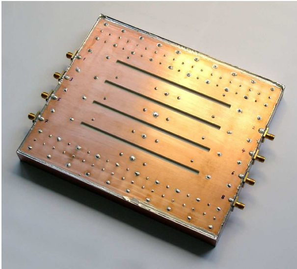
Figure 4: Slotline Electrode Model Beam Side
