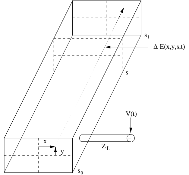
Figure 1: Basic Description of Pick-up or Kicker
