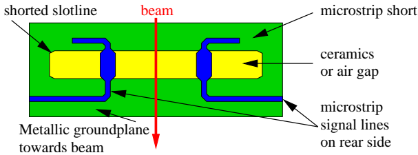
Figure 2: Conceptual Layout of Slotline Electrode
