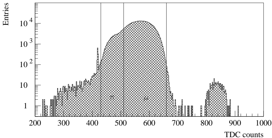
Fig. 11. The time of arrival of the beam cycle signal relative to the S1B scintillator for run 290, an ordinary run with no target. The graph corresponds to events where the digitised time from S1B was correct. The section labelled \mu contains those events used for the scattering analysis. The small peak to the right contains electrons. The resolution is slightly worse than in figure 9; this is not understood.
