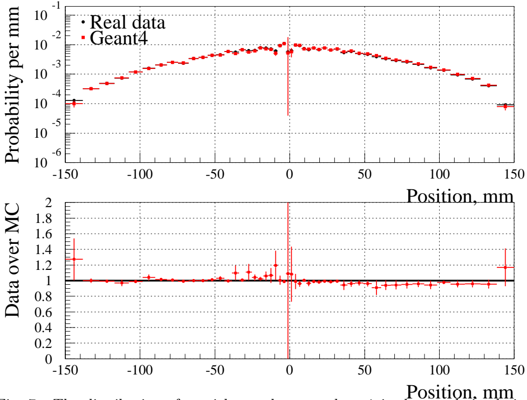
Fig. 7. The distribution of particles at detector plane 1 in data and simulation when the thick iron target is in place.
