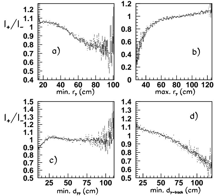
Figure 6: Data (points with error bars) - Monte Carlo (histogram) comparison of ratios I_+/I_- of normalized distance distributions between events with M_{00}^2 > (2m_+)^2 and M_{00}^2 < (2m_+)^2 (see text). a) min. r_\gamma : distance (cm) between LKr centre and closest photon; b) max. r_\gamma : distance (cm) between LKr centre and farthest photon; c) min. d_{\gamma\gamma} : minimum distance (cm) between photons at LKr; d) d_{\gamma\text{-track}} : minimum distance (cm) between photons and tracks at LKr.
