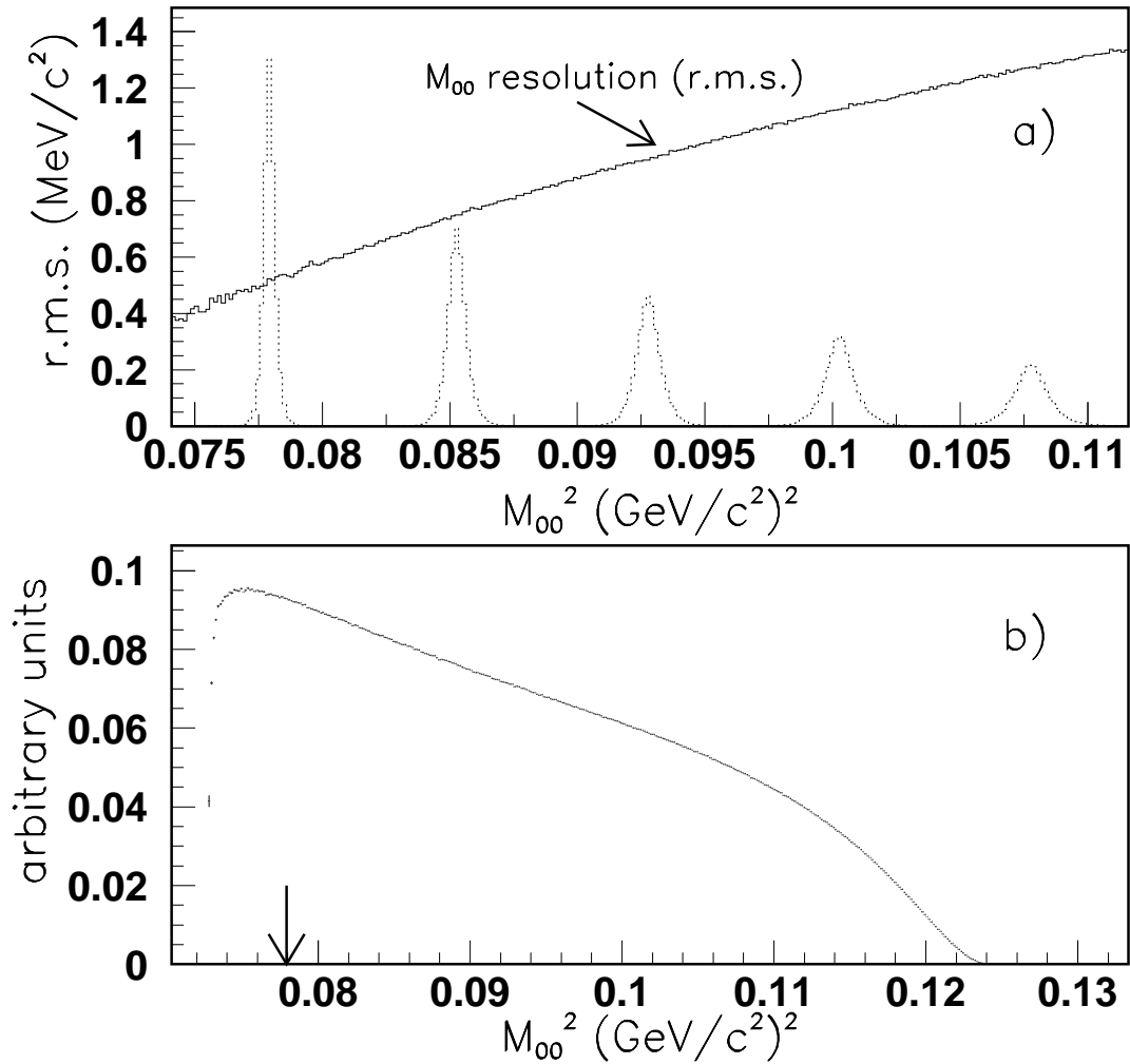
Figure 3: a) Expected M_{00} resolution (r.m.s. in \text{MeV}/c^2 ) versus generated M_{00}^2 (full line histogram), together with M_{00}^2 distributions for five generated values of M_{00}^2 ; b) Acceptance versus M_{00}^2 (see text). The point M_{00}^2 = (2m_+)^2 is indicated by the arrow.
