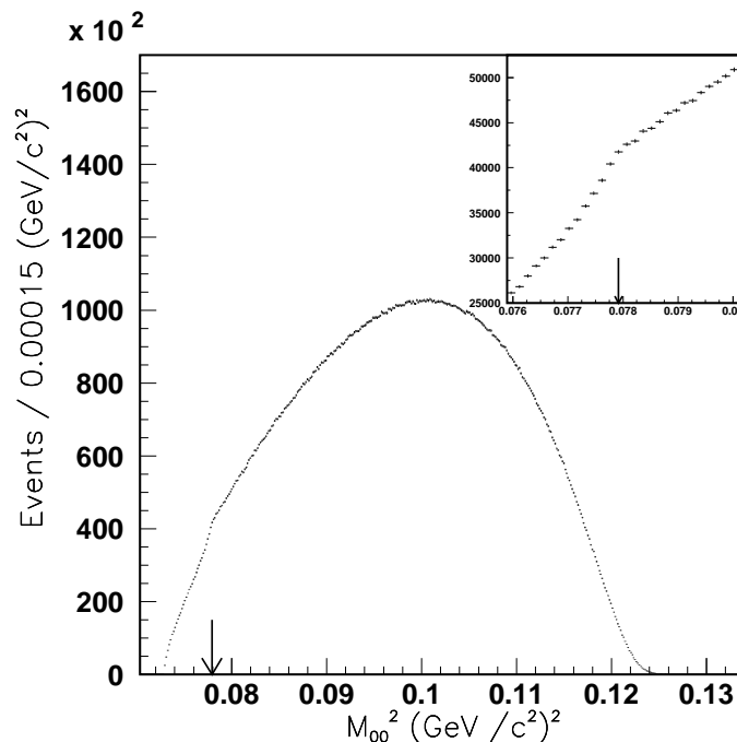
Figure 2: Distribution of M_{00}^2 , the square of the \pi^0\pi^0 invariant mass. The insert is an enlargement of a narrow region centered at M_{00}^2 = (2m_+)^2 (this point is indicated by the arrow). The statistical error bars are also shown in these plots.
