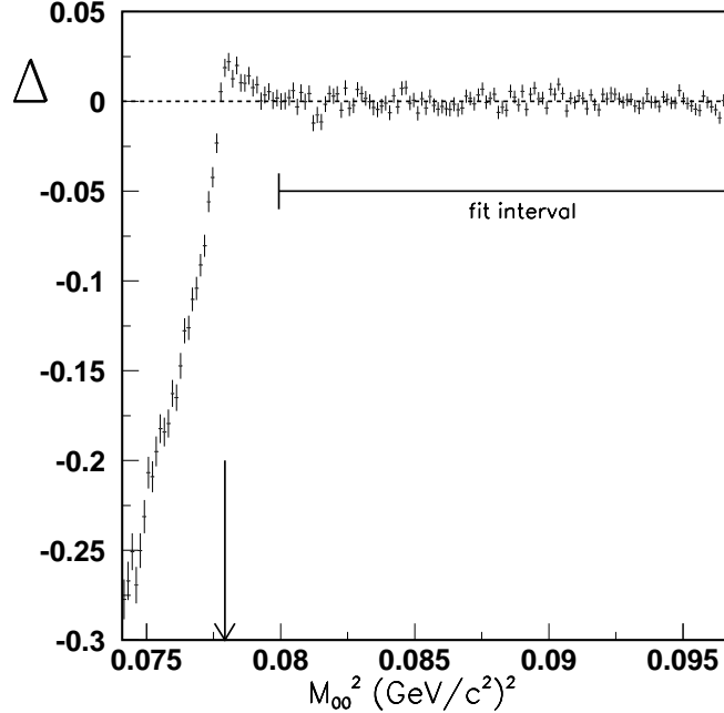
Figure 4: \Delta \equiv (data - fit)/data versus M_{00}^2 . The point M_{00}^2 = (2m_+)^2 is indicated by the arrow. Also shown is the M_{00}^2 region used in the fit.
