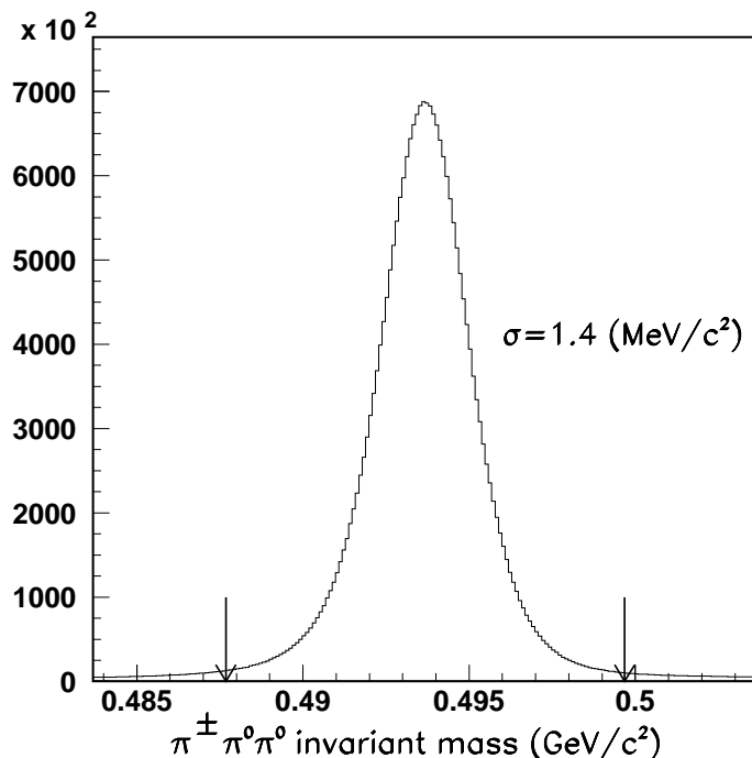
Figure 1: Invariant mass distribution of reconstructed \pi^\pm\pi^0\pi^0 candidate events. The arrows indicate the selected mass interval.
