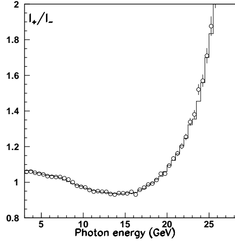
Figure 5: Data (points with error bars) - Monte Carlo (histogram) comparison of the ratio of normalized photon energy distributions I_+/I_- between events with M_{00}^2 > (2m_+)^2 and M_{00}^2 < (2m_+)^2 (see text)
