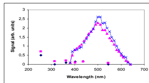
Fig.6. Spectra of the yellow stickers measure by a PMT. Rose squares - spectra of a “dark” sticker measured at wavelength corresponding to the strong lines from an Hg lamp, blue rhombus- the same measurements for a “light” sticker. Rose triangles – the reflective spectra of the “dark” sticker irradiated by a filament lamp, blue crosses- the same spectra measured for the “light” sticker
