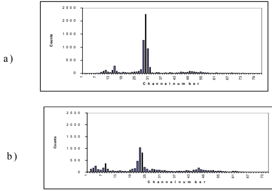
Fig. 7. On line digital image of the spectra of the yellow stickers (a-“light” and b-“dark”) measured with photosensitive RPC
