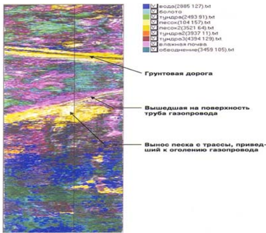
Fig2 A hyperspectroscopic computer synthesized image of the earth surface [1]. One can identify the surface composition, e.g. the yellow colour is sand, the rose colour is wheat earth, blue is water and the light blue represents swam.
