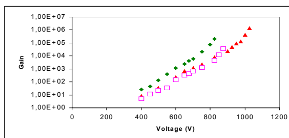
Fig. 15 Gain vs. voltage for RPCs and REHTA operating in mode B. Green rhombus – RPC combined with a semitransparent CsI photocathode, red triangles - REHTA combined with the semitransparent CsI photocathode, rose squares-REHTA combined with the CsTe/CsI photocathode. . All measurements were done in He+1%CH 4 +EF gas mixture [9].
