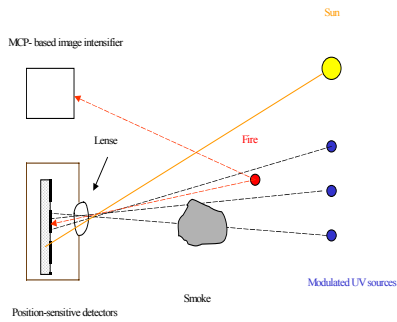
Fig.10. A schematic drawing of the experimental set up for visualization of the flames in the UV region of spectra and for detection of smoke
