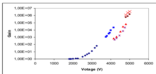
Fig. 14. Gain vs. voltage for the Cu coated G-10 hole type structure (blue) and for the REHTA operating in the mode A (red). Brown symbols represent the gain of the REHTA combined with an CsI photocathode. Gas mixture: Ar+5% isob =1 atm.
