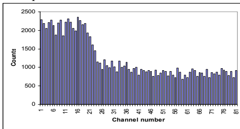
Fig. 8. On line digital image of a boarder between two yellow stickers measures with the RPC at 194 nm.
