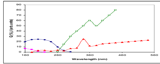
Fig. 12. The emission spectra of the flames in air (red) and the sun (green.) Rose the QE of the RPC combined with semitransparent CsI photocathode. Bleu- the QE of the CsTe photocathode [9]
