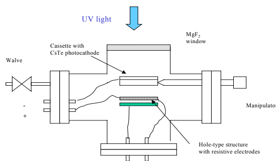
Fig. 16. A schematic drawing of the gas chamber for tests with CsTe photocathodes
