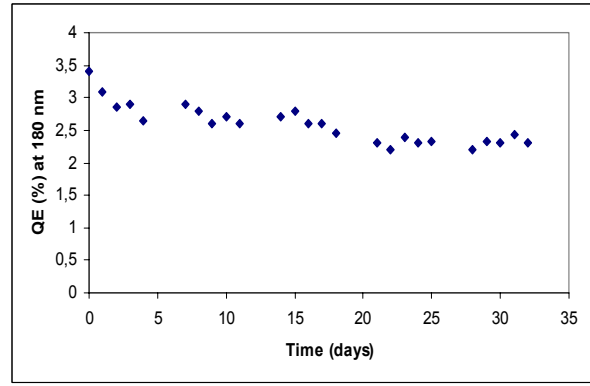
Fig. 9. Results of monitoring the RPCs QE with time
