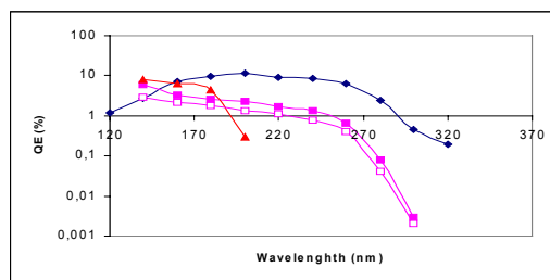
Fig. 17. QE of the photocathodes used in this work: bleu -QE of the CsTe photocathode measured in vacuum, rose filled squares QE of the CsTe photocathode in He+0,8%CH 4 +EF mixture [9], rose open squares-QE of the CsTe/CsI photocathode in He+0,8%CH 4 +EF; red triangles QE of the RPC combined with a CsI photocathode
