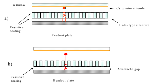
Fig. 13. A schematic drawing of the two designs of hole-type structures with resistive electrodes used in this work.
