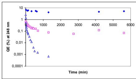
Fig. 18. QE vs. time for various photocathodes and at various conditions. Blue rhombus - QE of the CsTe photocathode installed in the gas chamber without a G-10 plate coated by graphite paint. Blue triangles- CsTe photocathode is combined with REHTA. Open rose squares - the same goes for an CsTe photocathode coated by a CsI protective layer. All measurements were done in He+0,8%CH 4 +EF gas mixture [9].
