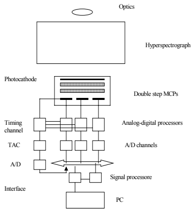
Fig1. A schematic drawing of the Reagent multianode MCP and the acquisition system
