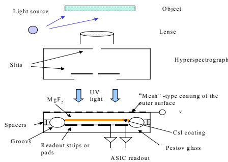
Fig.4. A schematic drawing of the experimental set up oriented on the spectroscopic and hyperspectroscopic measurements in the UV region of spectra
