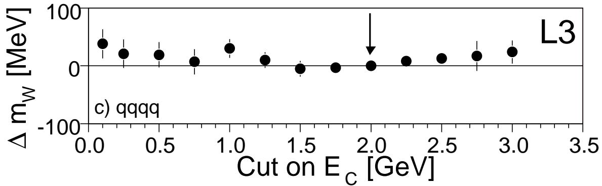
Figure 7: a) Energy spectrum of the clusters used in the jet reconstruction and changes of m_W for b) the qq\ell\nu and c) the qqqq final states caused by a variation of the cut on the minimum cluster energy, E_C . The arrows show the default values of the cut.
