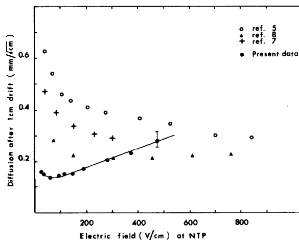
Fig. 6 - Electron diffusion as a function of the electric field in 80% Ar/20% CH 4 . Our measurement of the transverse component is compared to T.L. Cottrell et al. 8 in CH 4 . Also plotted is the measurement from F. Piuze 5 of the longitudinal diffusion in 80% Ar/20% CH 4 together with E.B. Wagner et al. 7 in CH 4 .
