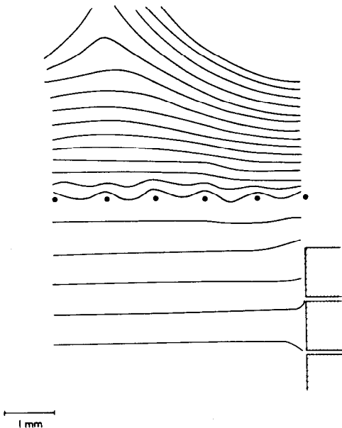
Fig. 2 - Equipotential lines at the junction between the converter stack and the pick-up chamber. The points represent the 100 \mu\text{m} diameter grid wires.
