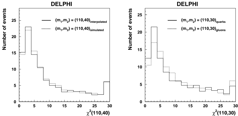
Figure 3: hA search. Left: distribution of \chi^2(110, 40) , as obtained from an interpolation between the nearest simulated samples at (m_h, m_A) = (110, 30) and (110, 50) \text{ GeV}/c^2 . It is compared with the true (dashed line) distribution from a simulated sample at (m_h, m_A) = (110, 40) . Right: distribution of \chi^2(110, 30) for Higgs bosons decaying into either q\bar{q} (solid line) or gg (dashed line), reflecting the worse mass resolution obtained for a four-gluon final state. In all distributions, overflows have been included in the last bin.
