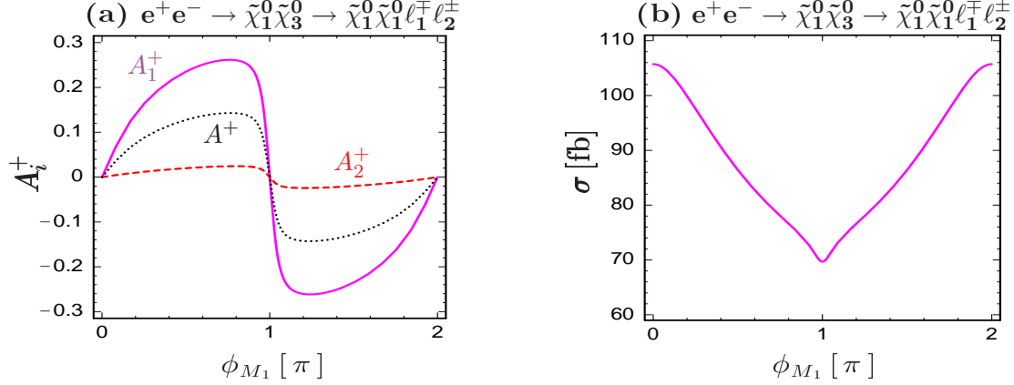
Figure 9: CP-odd asymmetries A_1^+ (solid), A_2^+ (dashed) and A^+ (dotted), Eqs. (47)–(49), for the process e^+e^- \rightarrow \tilde{\chi}_1^0\tilde{\chi}_3^0 \rightarrow \tilde{\chi}_1^0\tilde{\chi}_1^0\ell_1^\mp\ell_2^\pm and (b) the corresponding cross section as a function of \phi_{M_1} in scenario A, see Table 2, with \tan\beta = 3 . The centre-of-mass energy is \sqrt{s} = 500 GeV and the transverse beam polarizations are (\mathcal{P}_T^-, \mathcal{P}_T^+) = (100\%, 100\%) .
