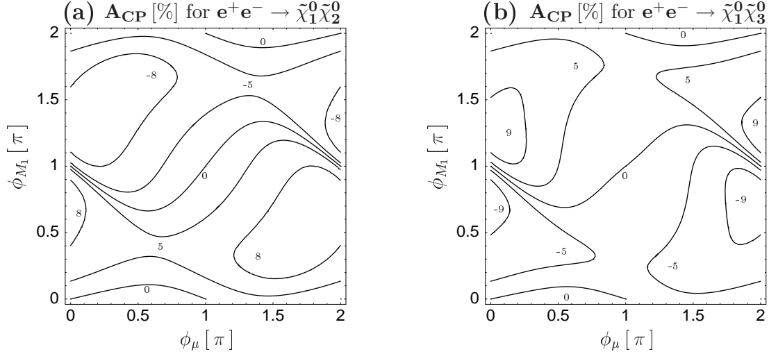
Figure 5: Contours of the CP asymmetry A_{CP} , Eq. (45), in % for the process (a) e^+e^- \rightarrow \tilde{\chi}_1^0 \tilde{\chi}_2^0 and (b) e^+e^- \rightarrow \tilde{\chi}_1^0 \tilde{\chi}_3^0 in the \phi_\mu - \phi_{M_1} plane, for scenario A with \tan\beta = 3 , see Table 2, for \sqrt{s} = 500 GeV and transverse beam polarizations (\mathcal{P}_T^-, \mathcal{P}_T^+) = (100\%, 100\%) .
