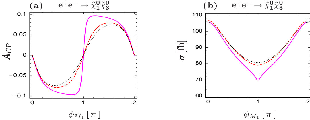
Figure 6: (a) CP asymmetry A_{CP} , Eq. (45), and (b) cross section \sigma(e^+e^- \rightarrow \tilde{\chi}_1^0 \tilde{\chi}_3^0) as a function of \phi_{M_1} for scenario A of Table 2, with \tan\beta = 3 (solid line), \tan\beta = 10 (dashed line), \tan\beta = 30 (dotted line), for \sqrt{s} = 500 GeV and transverse beam polarizations (\mathcal{P}_T^-, \mathcal{P}_T^+) = (100\%, 100\%) .
