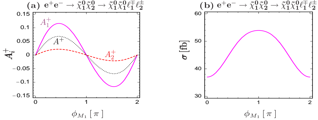
Figure 7: (a) CP-odd asymmetries A_1^+ (solid), A_2^+ (dashed) and A^+ (dotted), Eqs. (47)–(49), for the process e^+e^- \rightarrow \tilde{\chi}_1^0 \tilde{\chi}_2^0 \rightarrow \tilde{\chi}_1^0 \tilde{\chi}_1^0 \ell_1^\mp \ell_2^\pm and (b) the corresponding cross section as a function of \phi_{M_1} in scenario B (Table 2) with \tan \beta = 3 . The centre-of-mass energy is fixed at \sqrt{s} = 500 GeV and the transverse beam polarizations are (\mathcal{P}_T^-, \mathcal{P}_T^+) = (100\%, 100\%) .
