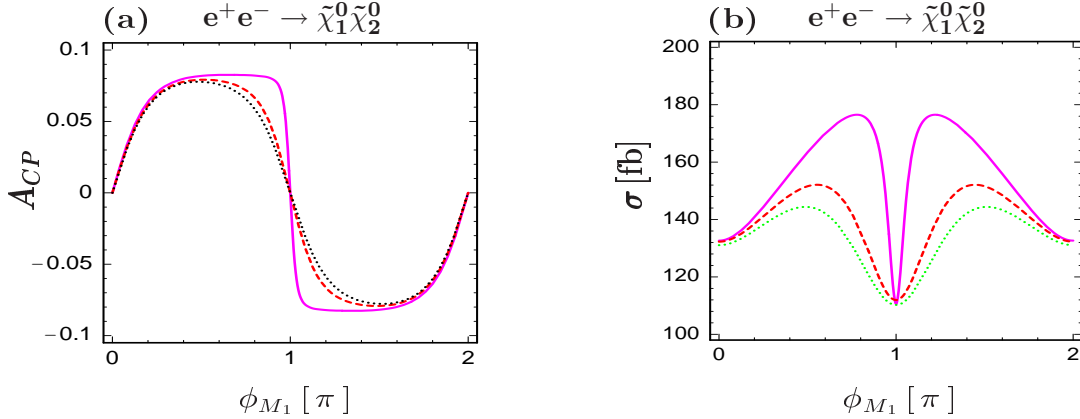
Figure 3: (a) CP asymmetry A_{CP} , Eq. (45), and (b) cross section \sigma(e^+e^- \rightarrow \tilde{\chi}_1^0 \tilde{\chi}_2^0) as a function of \phi_{M_1} for scenario A of Tab.2, with \tan\beta = 3 (solid line), \tan\beta = 10 (dashed line), \tan\beta = 30 (dotted line), for \sqrt{s} = 500 GeV and transverse beam polarizations (\mathcal{P}_T^-, \mathcal{P}_T^+) = (100\%, 100\%) .
