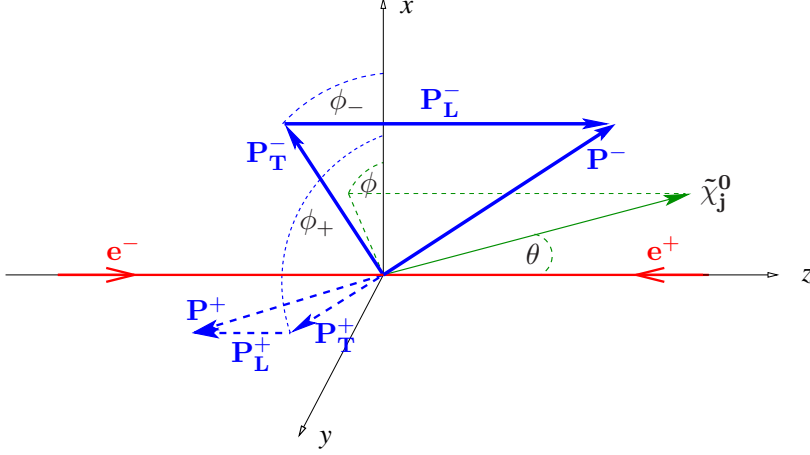
Figure 2: Decomposition of the e^\pm polarization vectors \mathbf{P}^\pm into the longitudinal components \mathbf{P}_L^\pm in the direction of the electron/positron momentum and the transverse components \mathbf{P}_T^\pm = \mathcal{P}_T^\pm \vec{t}_\pm with respect to a fixed coordinate system (x, y, z) . The z -axis is in the direction of the electron momentum.
