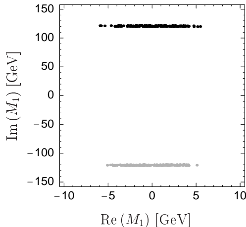
Figure 10: SUSY parameter points in the \text{Re}(M_1) – \text{Im}(M_1) plane consistent with scenario B, if one assumes an uncertainty of 1% for the masses and 1\text{-}\sigma deviation ( \mathcal{L}_{\text{int}} = 100 \text{ fb}^{-1} ) for the cross sections and the asymmetry. The parameters |M_1| , \phi_{M_1} , M_2 , |\mu| , \phi_\mu and \tan\beta have been randomly scanned around the reference point B. The grey points are excluded if one takes into account the CP-odd observable A_{CP} , Eq. (45).
