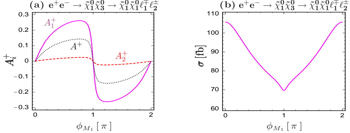
Figure 9: CP-odd asymmetries A_1^+ (solid), A_2^+ (dashed) and A^+ (dotted), Eqs. (47)–(49), for the process e^+e^- \rightarrow \tilde{\chi}_1^0 \tilde{\chi}_3^0 \rightarrow \tilde{\chi}_1^0 \tilde{\chi}_1^0 \ell_1^\mp \ell_2^\pm and (b) the corresponding cross section as a function of \phi_{M_1} in scenario A, see Table 2, with \tan\beta = 3 . The centre-of-mass energy is \sqrt{s} = 500 GeV and the transverse beam polarizations are (\mathcal{P}_T^-, \mathcal{P}_T^+) = (100\%, 100\%) .
