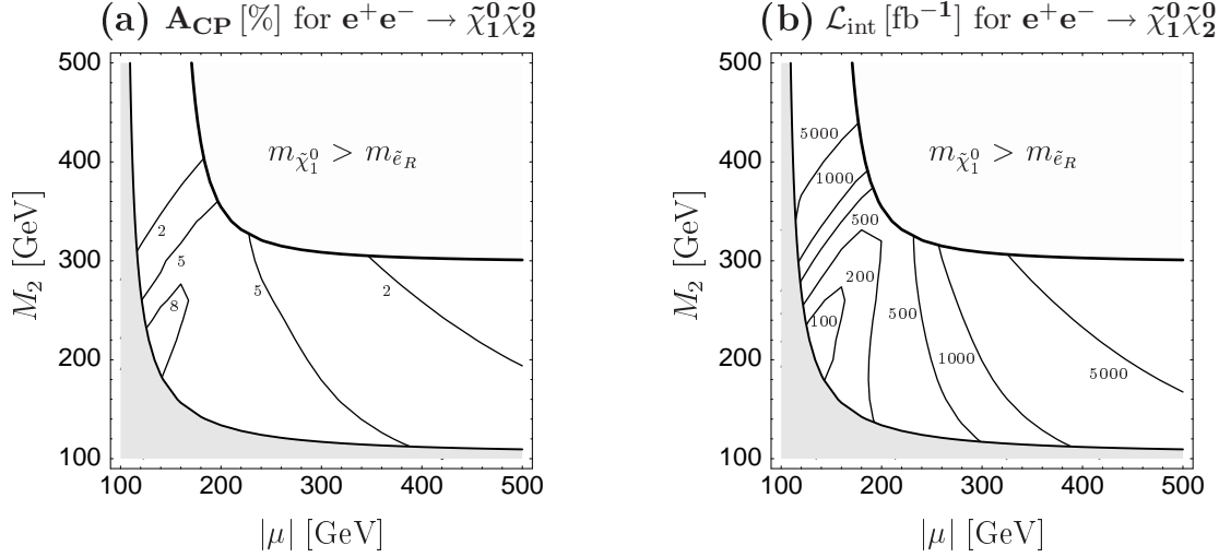
Figure 4: (a) contours of the CP asymmetry A_{CP} , Eq. (45), in % for the process e^+e^- \rightarrow \tilde{\chi}_1^0 \tilde{\chi}_2^0 in the |\mu|-M_2 plane. The MSSM parameters are \phi_{M_1} = 0.5\pi , \phi_\mu = 0 , \tan\beta = 3 , m_{\tilde{e}_L} = 400 GeV and m_{\tilde{e}_R} = 150 GeV at \sqrt{s} = 500 GeV with transverse beam polarizations (\mathcal{P}_T^-, \mathcal{P}_T^+) = (100\%, 100\%) . (b) shows the contours of the luminosity \mathcal{L}_{\text{int}} , Eq. (51), needed to measure the CP-odd asymmetry A_{CP} at the 5- \sigma level with degrees of transverse polarization (\mathcal{P}_T^-, \mathcal{P}_T^+) = (80\%, 60\%) . The light-grey region is experimentally excluded by the exclusion bound m_{\tilde{\chi}_1^\pm} < 104 GeV [28].
