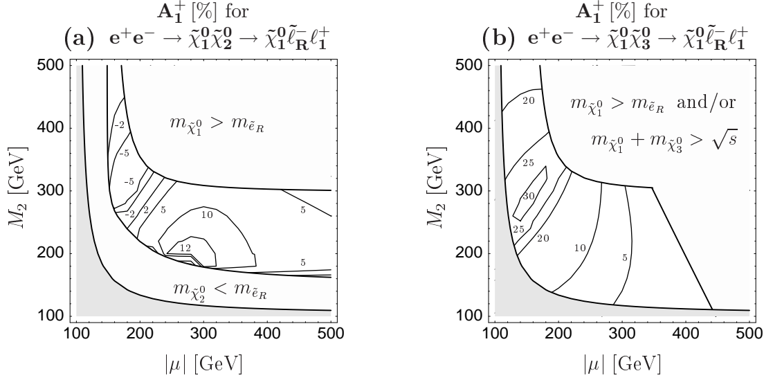
Figure 8: Contours of the CP-odd asymmetry A_1^+ , Eq. (47), in % in the |\mu| - M_2 plane for the process (a) e^+e^- \rightarrow \tilde{\chi}_1^0 \tilde{\chi}_2^0 \rightarrow \tilde{\chi}_1^0 \tilde{\ell}_R^- \ell_1^+ and (b) e^+e^- \rightarrow \tilde{\chi}_1^0 \tilde{\chi}_3^0 \rightarrow \tilde{\chi}_1^0 \tilde{\ell}_R^- \ell_1^+ . The MSSM parameters are \phi_{M_1} = 0.5\pi , \phi_\mu = 0 , \tan\beta = 3 , m_{\tilde{e}_L} = 400 GeV and m_{\tilde{e}_R} = 150 GeV. The centre-of-mass energy is fixed at \sqrt{s} = 500 GeV and the transverse beam polarizations are (\mathcal{P}_T^-, \mathcal{P}_T^+) = (100\%, 100\%) . The light-grey region is excluded by m_{\tilde{\chi}_1^\pm} < 104 GeV [28].
