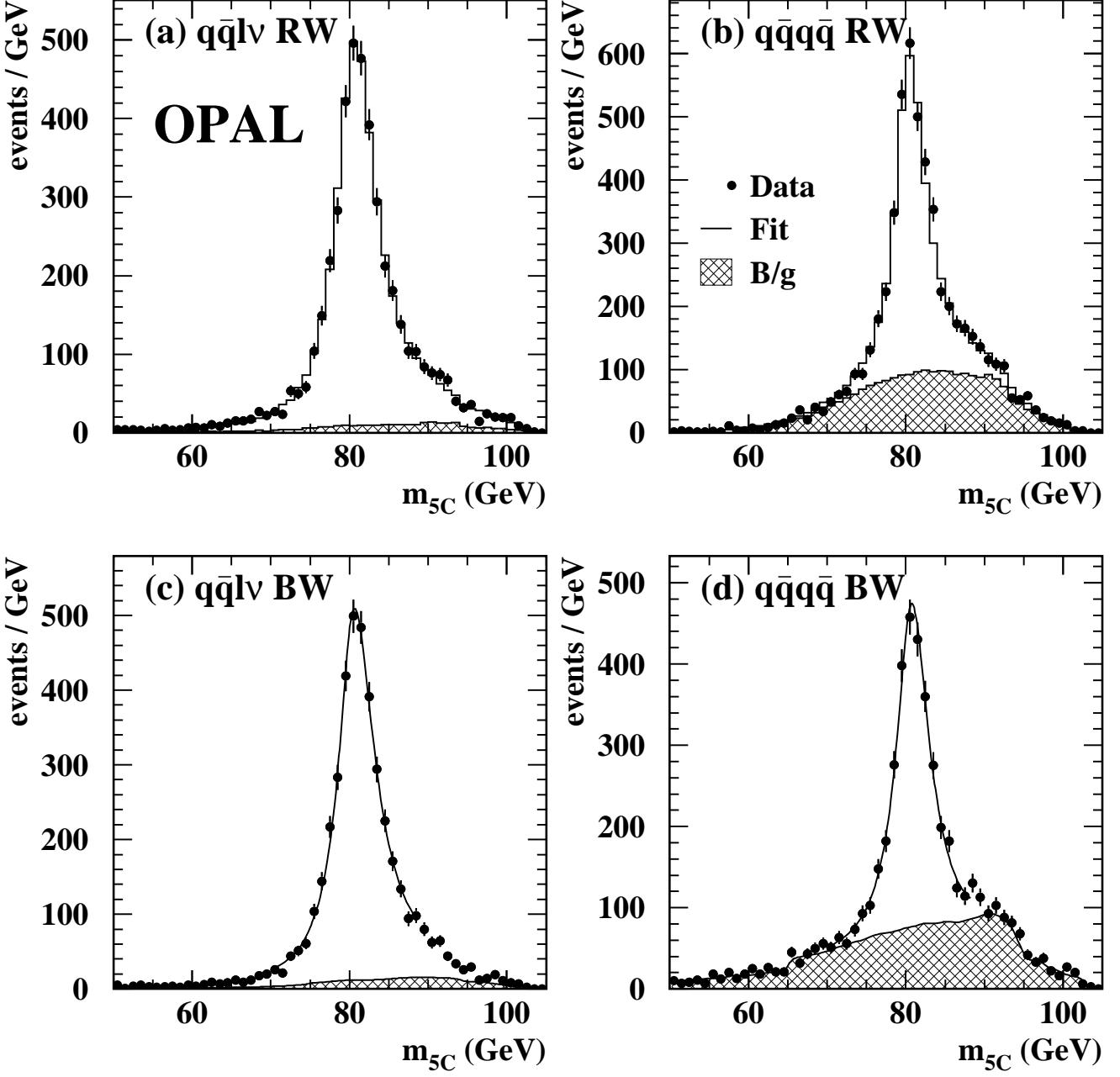
Figure 7: Distributions of 5C fit masses for the q\bar{q}l\nu and q\bar{q}q\bar{q} channels in the reweighting (a,b) and Breit-Wigner (c,d) fits. For the reweighting fits, the histograms show the reweighted template distributions corresponding to the fitted W mass values, and for the Breit-Wigner fits, the fitted functions are indicated by the solid lines drawn over the fit regions (70–88 GeV). In both cases, the estimated background contributions are indicated by the shaded regions.
