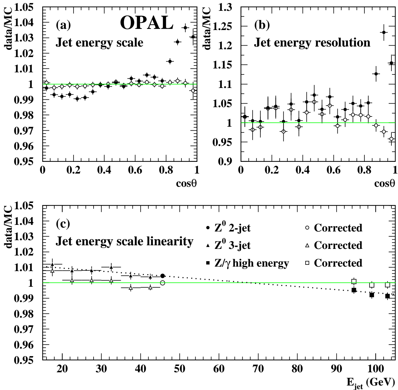
Figure 8: Determination of energy corrections for jets (see text). Ratios of data to Monte Carlo are shown averaged over all data-taking years for: (a) jet energy scale as a function of \cos\theta , (b) jet energy resolution as a function of \cos\theta , (c) jet energy scale as a function of the jet energy itself. The results using the uncorrected simulation are shown by the filled points, and those with the corrected simulation are shown by the open points, with the error bars indicating the statistical error in each case. The horizontal lines indicate ratios of unity, and the dotted line in (c) shows the linearity correction used to parameterise the jet energy scale dependence on the jet energy itself.
