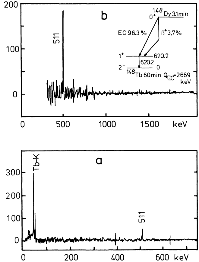
Fig. 4 Quanta spectrum of ^{148}\text{Dy} gated by 620 keV transitions, a) low energy, b) high energy part. Inset: decay scheme of ^{148}\text{Dy}
