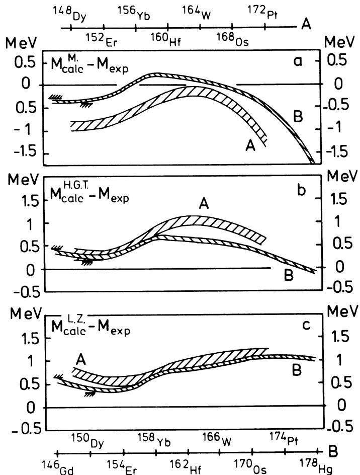
Fig. 6 a-c Comparison of experimental results of Table 2 with predictions of current mass formulae, mass differences in MeV, a) calculated masses of Myers, b) of Hilf et al., c) of Liran and Zeldes
