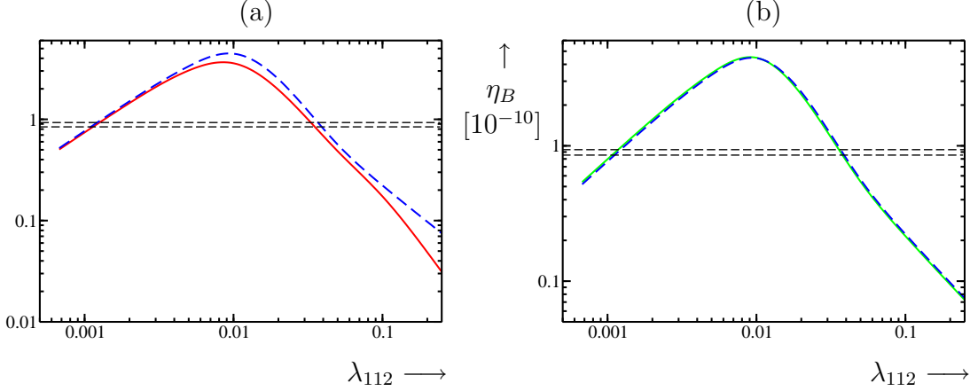
Figure 3: (a) The baryon asymmetry in units of 10^{-10} as function of \lambda_{112} for m_{\tilde{u}} = 1 \times 10^{13} GeV, \lambda_{123} = 0.25 , k_{q_1} = 1 , \theta_{13} = 0.1 and m_{\tilde{d}_3}^2/m_{\tilde{u}}^2 = 10 . The full (dashed) line includes (neglects) scatterings. (b) The baryon asymmetry with (without) a light \tilde{q}_1 in solid (dashed) line. Scatterings are neglected.
