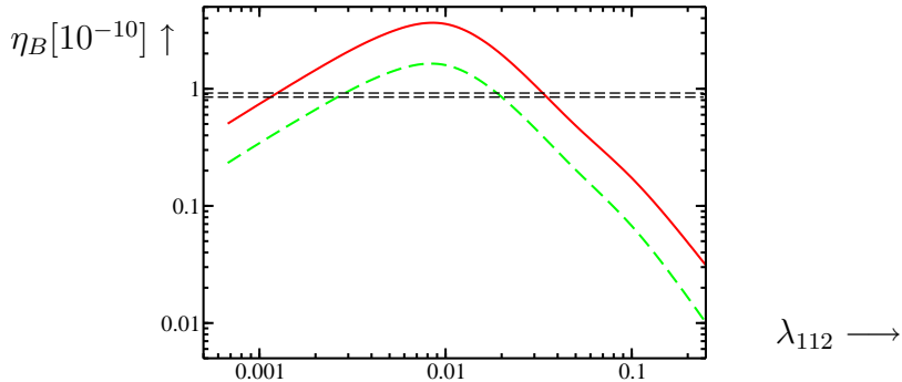
Figure 4: The baryon asymmetry in units of 10^{-10} as function of \lambda_{112} for m_{\tilde{u}} = 1 \times 10^{13} GeV, k_{q1} = 1 , \theta_{13} = 0.1 and m_{d_3}^2/m_{\tilde{u}}^2 = 10 . Solid (dashed) lines indicate \lambda_{123} = 0.25 (0.1). Scatterings are included.
