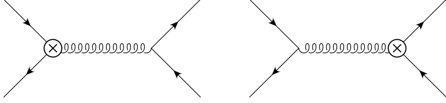
Figure II.2: Counterterm diagrams.
