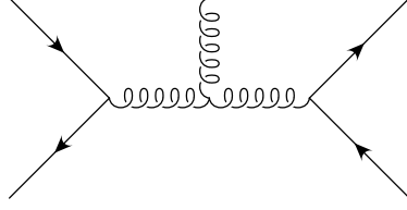
Figure III.2: Amplitude containing the triple gluon vertex. The diagram does not contribute here because of the colour structure.
