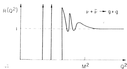
Fig. 2. Hypothetical cross section for the process \nu + \bar{\nu} \rightarrow \text{hadrons} (gluonia) in pure quarkless QCD, normalized to the point cross section.
