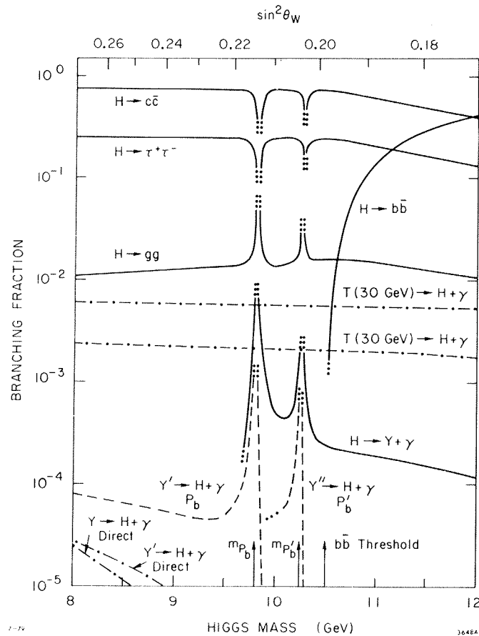
Fig. 1. Properties of a standard model Higgs-boson of mass ~10 GeV (the "scalon"). Taken from Ref. 35).
