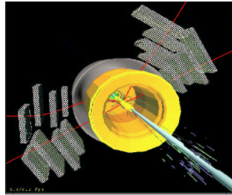
Figure 2: Higgs event displayed by IGUANACMS
