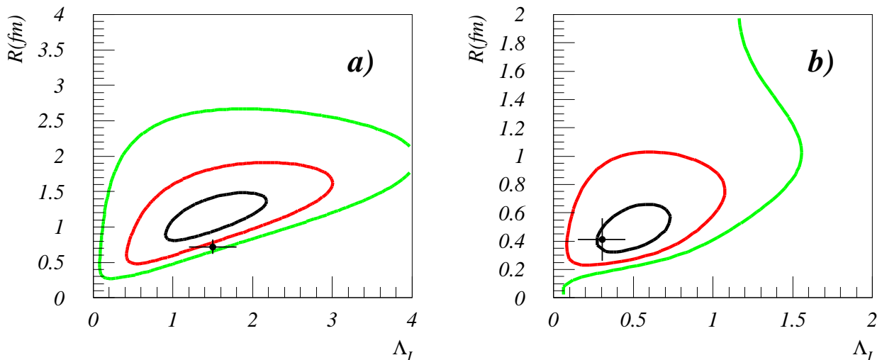
Figure 9: The 2-d \Delta\chi^2 curves are shown for \Lambda_I and R . (a) shows the results for like-sign pairs, while in (b) the unlike-sign pair result is displayed. The three contours correspond to a \Delta\chi^2 of 1, 4, and 9 respectively. The crosses show the prediction from LUBOEI BE 32 . The errors corresponding to the LUBOEI predictions are multiplied by a factor 5 for clarity.
