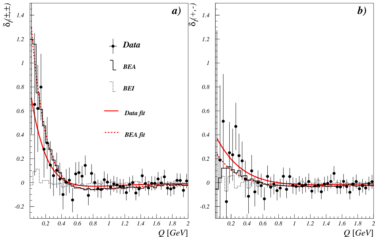
Figure 8: The \delta_I(Q) distribution for like-sign (a) and unlike-sign (b) particle pairs. The BE 32 models including BEC between all particle pairs and pairs coming from the same W only are superimposed on the plots, together with the fit results using equation (12). The fit results are with fixed R and \epsilon_d and are corrected for the bias mentioned in section 6.4.
