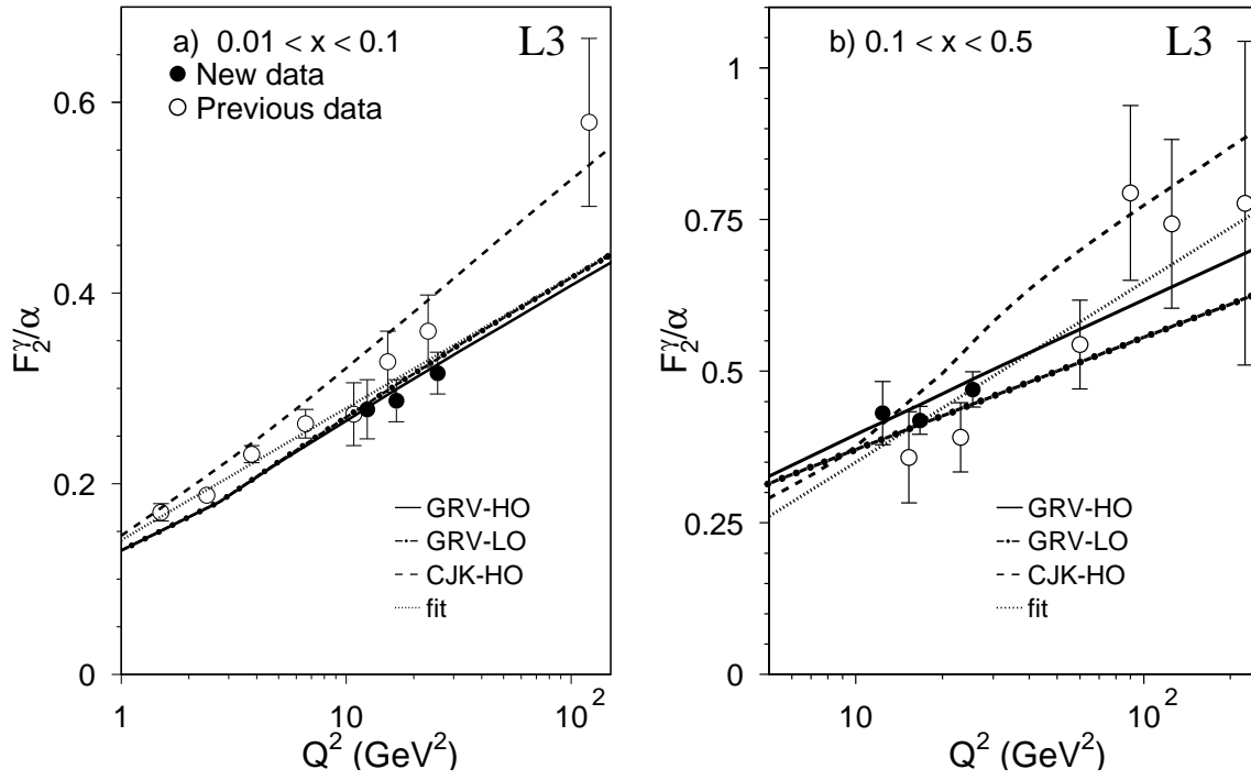
Figure 7: Evolution of the photon structure function F_2^\gamma/\alpha as a function of Q^2 for two x intervals. The results of a fit to the data of the function a + b(\ln Q^2 / \text{GeV}^2) are shown together with the predictions of the higher-order parton density functions GRV and CJK as well as the leading-order predictions of GRV.
