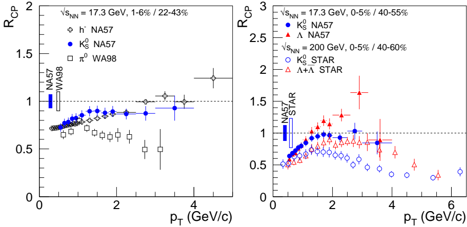
Fig. 4. (colour online) Left: R_{CP}(p_T) for h^- and K_S^0 from NA57 and \pi^0 from WA98 [7] in Pb–Pb collisions at \sqrt{s_{NN}} = 17.3 GeV. Right: R_{CP}(p_T) for K_S^0 and \Lambda in Pb–Pb at \sqrt{s_{NN}} = 17.3 GeV (NA57) and in Au–Au at \sqrt{s_{NN}} = 200 GeV (STAR) [2]; slightly different peripheral classes are employed for the comparison. The bars centered at R_{CP} = 1 represent the normalization errors; the point-by-point bars are the quadratic sum of statistical and systematic errors.
