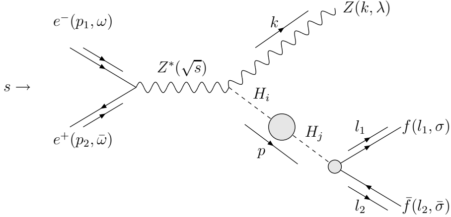
Figure 1: The dominant mechanism contributing to the process e^+e^- \rightarrow H_i Z \rightarrow [f(\sigma)\bar{f}(\bar{\sigma})] Z .
