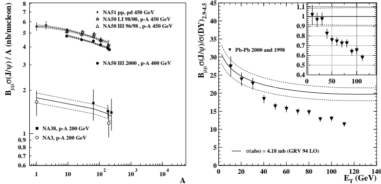
Figure 1: Simultaneous Glauber fit using the ratio B_{\mu\mu}\sigma(J/\psi)/A to extract the J/\psi rescaling factors (left panel). The ratios J/\psi/DY in Pb-Pb are compared with the nuclear absorption curve as a function of E_T (right panel).
