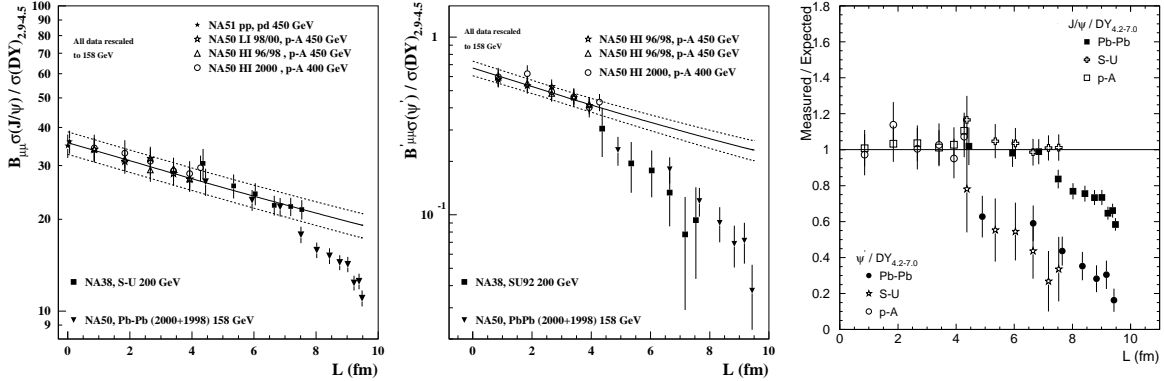
Figure 2: The ratios J/\psi/DY as a function of L (left panel) and \psi'/DY as a function of L (center panel). The same ratios divided by the expected values deduced from p-A collisions (right panel).
