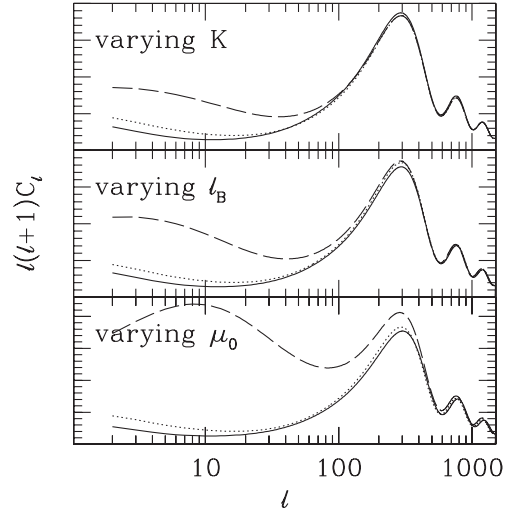
FIG. 2. The effect of the MOND parameters on the power of spectrum of the CMB. Top panel: \mu_0 = 200 , l_B = 100 Mpc, and K = 1 (solid), 0.1 (dotted), and 0.08 (dashed); Middle panel: \mu_0 = 200 , K = 0.1 , and l_B = 1000 Mpc (solid), 100 Mpc (dotted), and 10 Mpc (dashed); Bottom panel: K = 0.1 , l_B = 100 Mpc, and \mu_0 = 1000 (solid), 200 (dotted), and 150 (dashed).
