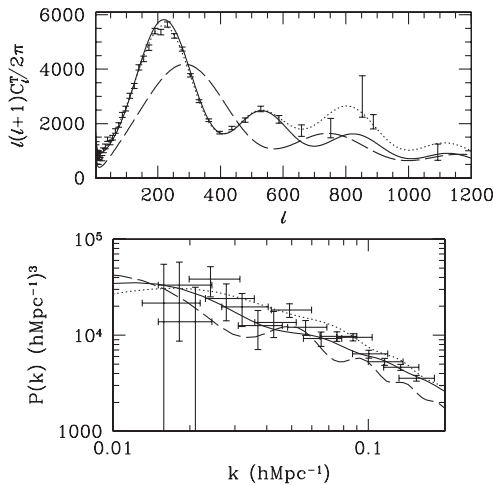
FIG. 4. The angular power spectrum of the CMB (top panel) and the power spectrum of the baryon density (bottom panel) for a MOND universe (with a_0 \approx 4.2 \times 10^{-8} cm/s 2 ) with \Omega_\Lambda = 0.78 and \Omega_\nu = 0.17 and \Omega_B = 0.05 (solid line), for a MOND universe \Omega_\Lambda = 0.95 and \Omega_B = 0.05 (dashed line) and for the \Lambda CDM model (dotted line). A collection of data points from CMB experiments and Sloan are overplotted.
