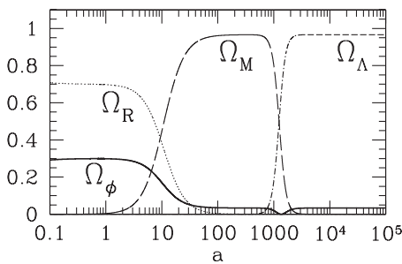
FIG. 1. The relative energy densities in \phi (thick solid line), radiation (dotted line), matter (dashed line), and \Lambda (dot-dashed line) for \mu_0 = 5 as a function of the scale factor ( a is in arbitrary units). Note that the energy density in the scalar field tracks the dominant form of energy at each instance in time.
