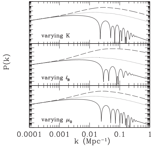
FIG. 3. The effect of the MOND parameters on the power of spectrum of the baryonic density fluctuations. Top panel: \mu_0 = 200 , l_B = 100 Mpc, and K = 1 (solid), 0.1 (dotted), and 0.08 (dashed); Middle panel: \mu_0 = 200 , K = 0.1 , and l_B = 1000 Mpc (solid), 100 Mpc (dotted), and 10 Mpc (dashed); Bottom panel: K = 0.1 , l_B = 100 Mpc, and \mu_0 = 1000 (solid), 200 (dotted), and 150 (dashed).
