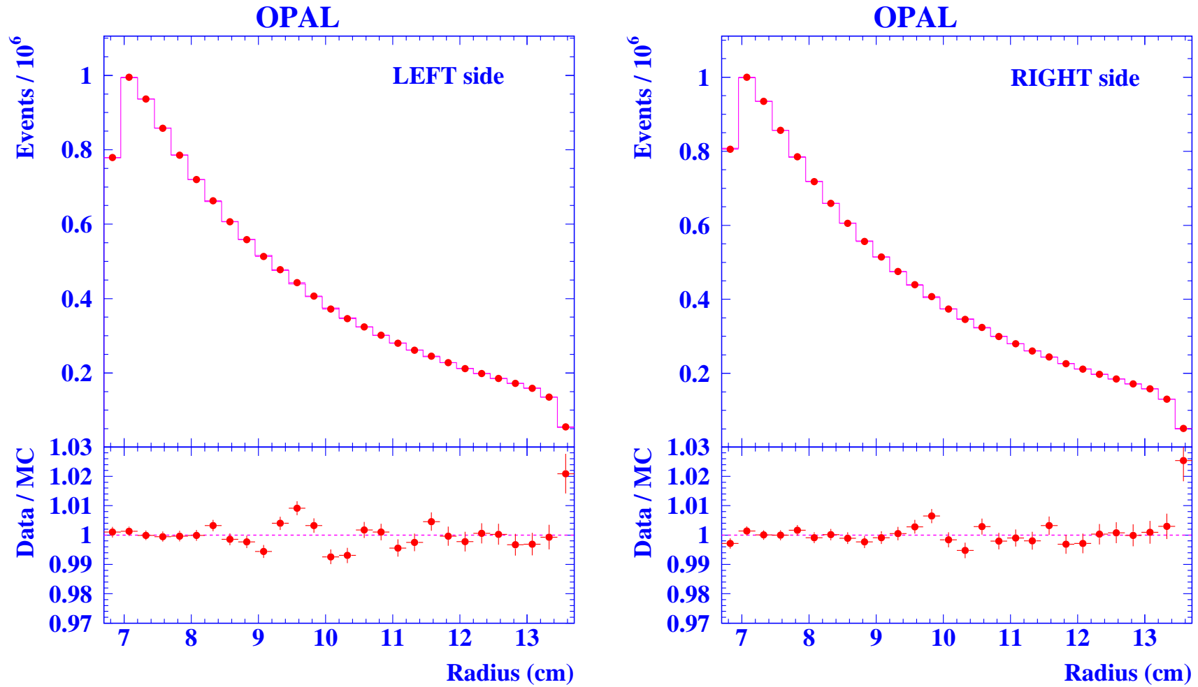
Figure 2: Radial distributions after the isolation cuts for the complete data statistics in the Left and Right calorimeters (mean \sqrt{s} = 91.2208 GeV). The points show the data and the histogram the Monte Carlo prediction, assuming the expected running of \alpha , normalized to the same number of events. The lower plots show the ratio between data and Monte Carlo.
