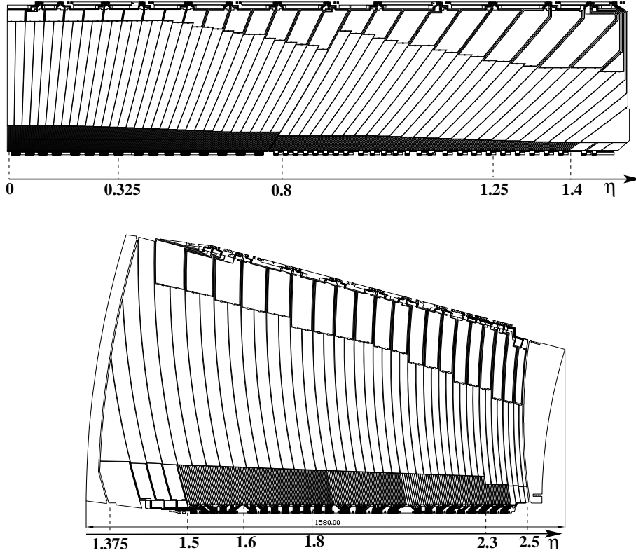
Fig. 1. Segmentation of barrel and end-cap electrodes.
