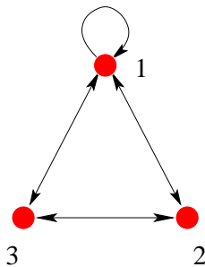
Figure 4: The quiver for the SPP theory.
