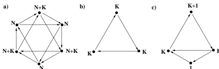
Figure 14: Quiver diagrams for the theory with K fractional branes of the (1, 0, 1, 0, 1, 0) kind, at a generic point in the cascade (figure a ), and in the infrared (figure b ). Figure c shows the infrared limit of the same theory with one additional fractional brane of the (1, 0, 0, 1, 0, 0) kind.
