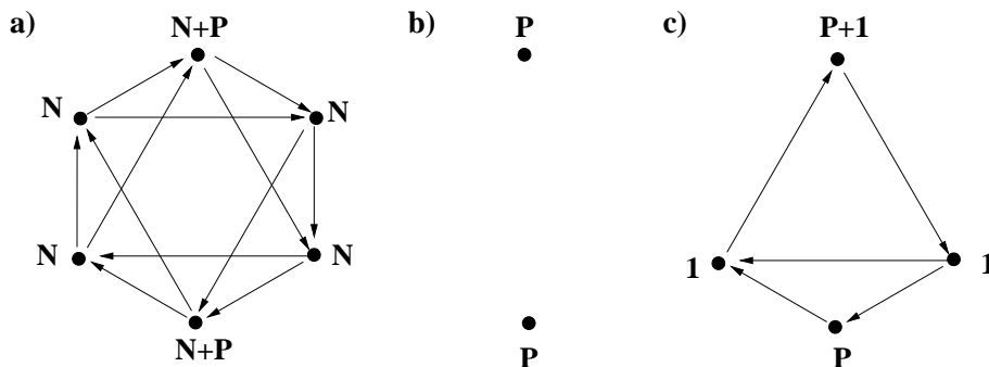
Figure 13: Quiver diagrams for the theory with P fractional branes of the (1, 0, 0, 1, 0, 0) kind, at a generic point in the cascade (figure a ), and in the infrared limit (figure b ). Figure c shows the infrared limit of the same theory with an additional fractional brane of the (1, 0, 1, 0, 1, 0) kind.
