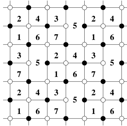
Figure 25: Brane tiling for model I of PdP_4 .
