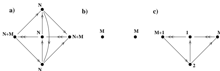
Figure 10: Figures (a) shows the quiver theory describing dP_2 with N D3-branes and M fractional branes of the (1, 1, 0, 0, 0) kind, while figure (b) shows the quiver for the infrared limit of the corresponding duality cascade. Figure (c) shows the addition of a fractional D-brane probe of the (1, 0, 1, 0, 2) kind to that theory.
