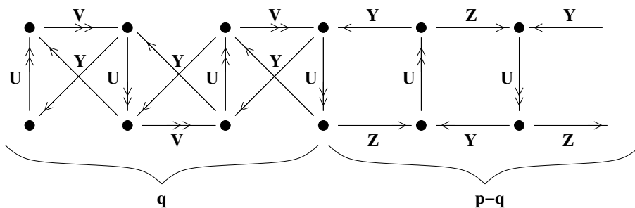
Figure 20: General picture of the toric phase of Y^{p,q} that we are considering.
