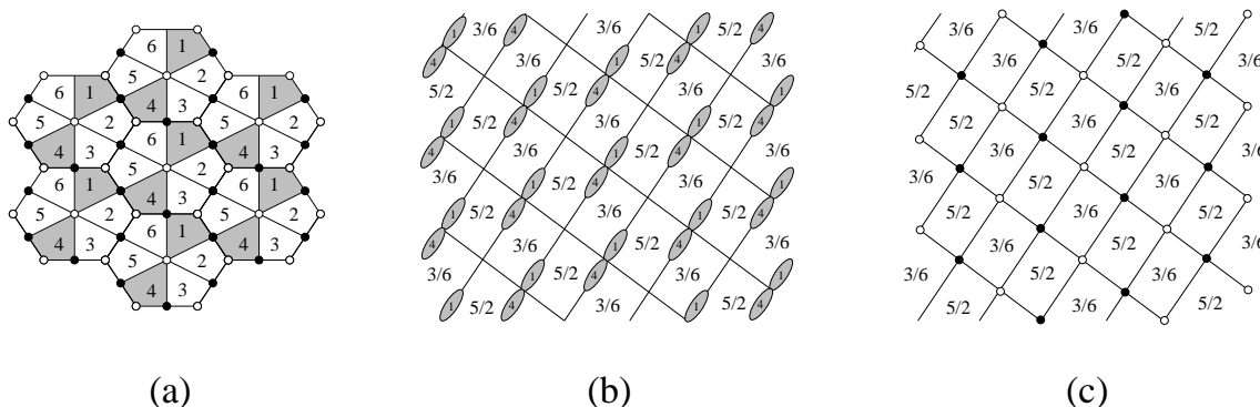
Figure 22: a) Brane tiling for the (1, 0, 0, 1, 0, 0) deformation fractional brane of model I of dP_3 . b) and c) Complex deformation to the conifold.
