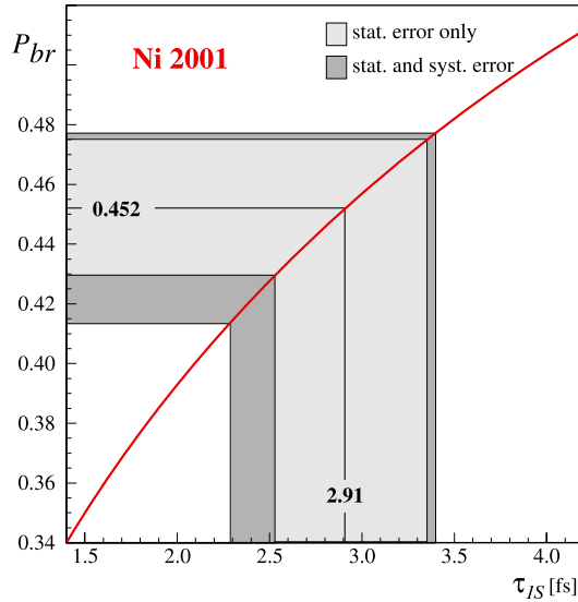
Fig. 6. Break-up probability P_{br} as a function of the lifetime of the atomic ground state \tau_{1S} for the combined 94 and 98 \mu\text{m} thick Ni targets. The experimentally determined P_{br} with statistical and total errors translates into a value of the lifetime with corresponding errors.
