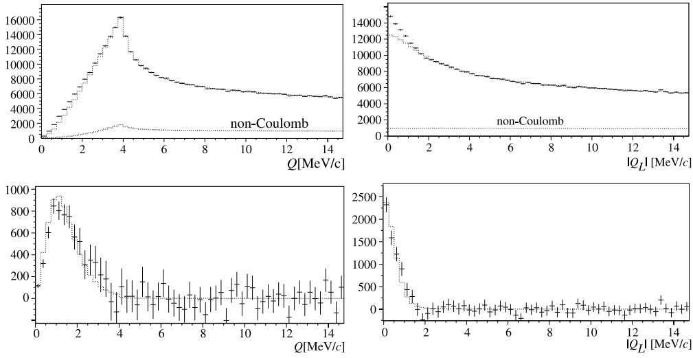
Fig. 3. Top: Experimental Q and Q_L distributions after subtraction of the prompt accidental background, and fitted Monte Carlo backgrounds (dotted lines). The peak at Q = 4 \text{ MeV}/c is due to the cut Q_T \leq 4 \text{ MeV}/c . Bottom: Residuals after background subtraction. The dotted lines represent the expected atomic signal shape. The bin-width is 0.25 \text{ MeV}/c .
