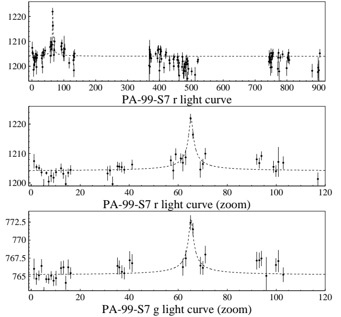
Fig. 6. 3-year light curves of the microlensing event PA-99-S7. Panels and symbols as in Figure 4.
