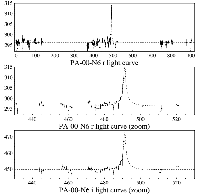
Fig. 5. 3-year light curves of the microlensing event PA-00-N6. Panels and symbols as in Figure 4.
