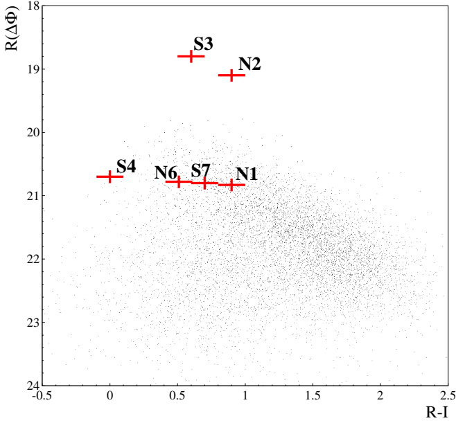
Fig. 7. R(\Delta\Phi) ( R-I ) colour-magnitude diagram for the 10 000 variations selected before the cut on the flux deviation at maximum. Superimposed we show the positions of the 6 selected candidates. The R-I colours for PA 99-N2 and PA 99-S7 are estimates derived from the observed V-R colours.
