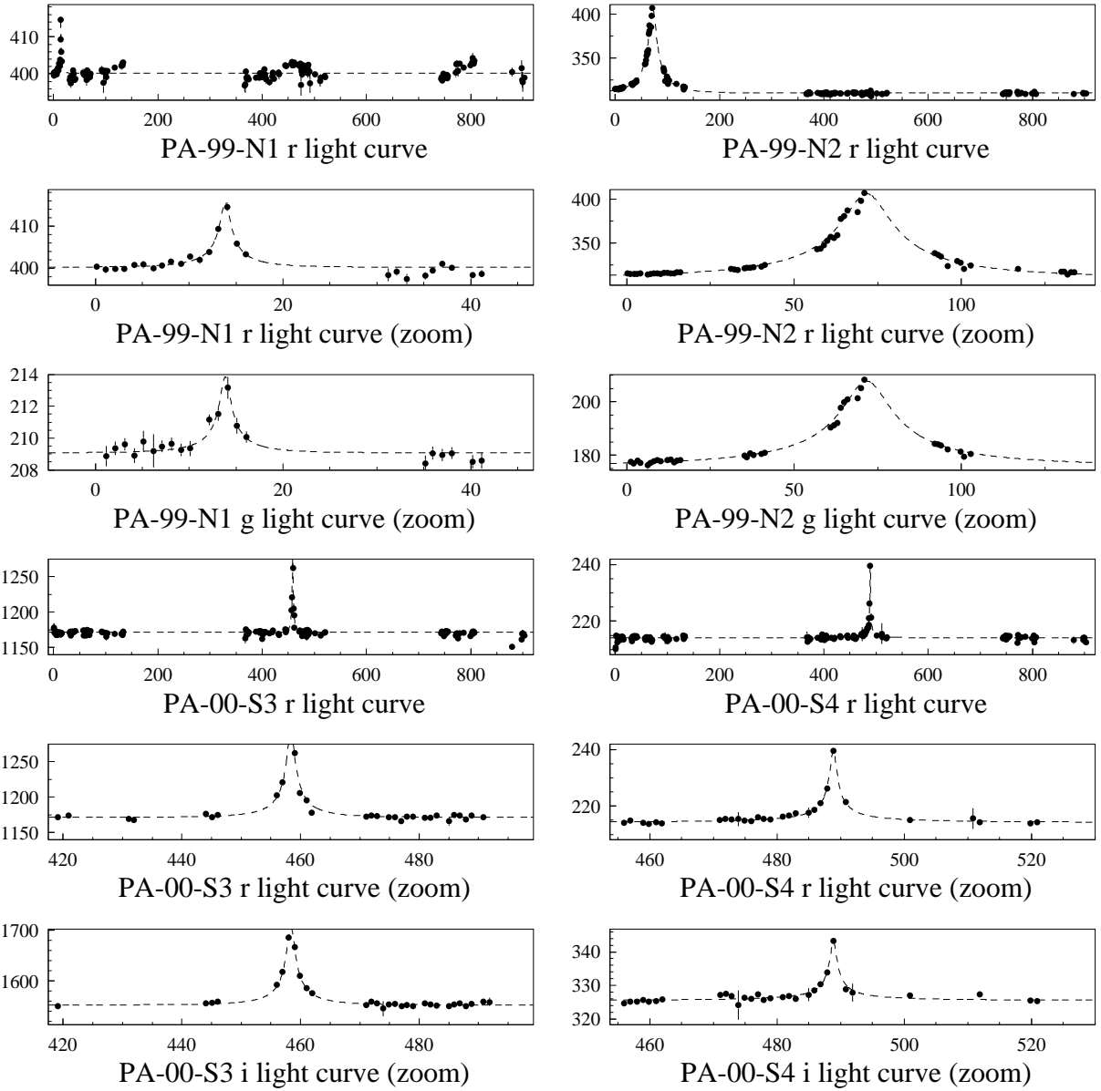
Fig. 4. 3-year light curves of the four microlensing events PA-99-N1, PA-99-N2, PA-00-S3 and PA-00-S4. For each event, the top panel shows the whole light curve in the r filter, while the 2 lower panels display zoomed light curves in all bands for which data are available. Dashed lines are best-fit Paczyński curves. The abscissae are time in days (JD-2451392.5). The ordinates are flux in ADU/s.
