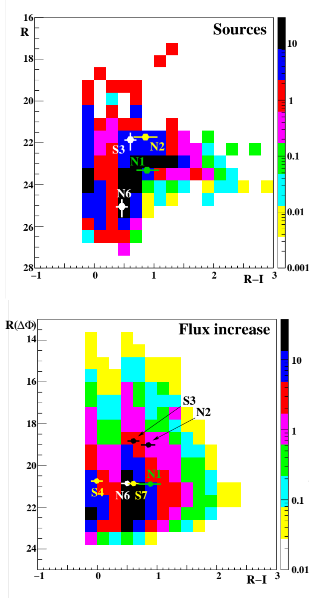
Fig. 9. The colour/magnitude event density distribution predicted by the Monte Carlo. Top panel: R magnitude of the source star. Bottom panel: R magnitude of the flux increase. The observed events are superposed on the diagrams. Only those events for which the source magnitude can be reliably extracted appear in the left panel. The colour scale shows the event density (in arbitrary units).
