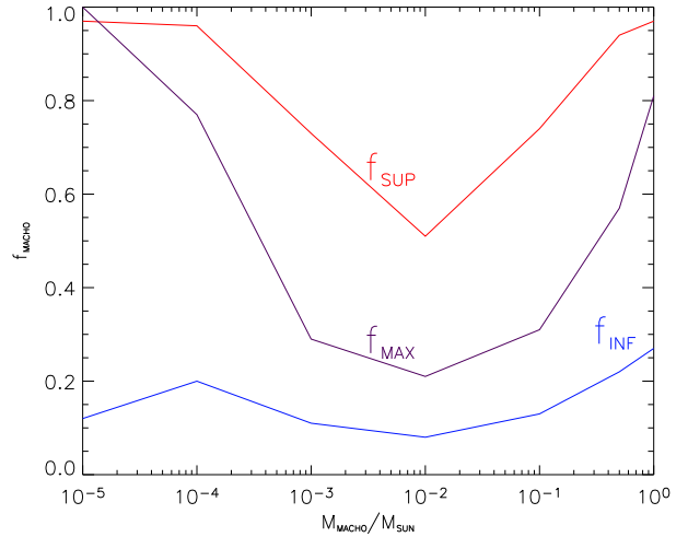
Fig. 12. Most probable value, upper and lower 95% CL limit for the halo fraction as a function of the MACHO mass for a_{M31} = 3 \text{ kpc} and stellar bulge (disc) M/L_B = 3 (4).
