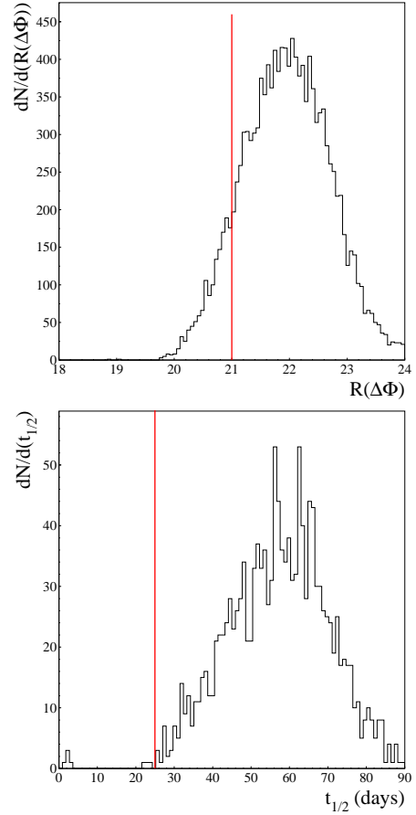
Fig. 2. Top: Distribution of flux deviations at maximum for the selected events after the sampling cut. Bottom: Duration distribution for the selected events after the cut on R(\Delta\Phi) .
