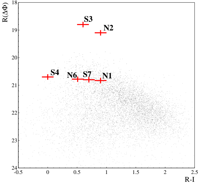
Fig. 7. R(\Delta\Phi) - (R - I) colour-magnitude diagram for the \sim 10\,000 variations selected before the cut on the flux deviation at maximum. Superimposed we show the positions of the 6 selected candidates. The R - I colours for PA - 99 - N2 and PA - 99 - S7 are estimates derived from the observed V - R colours.
