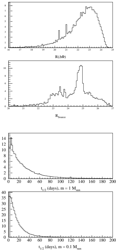
Fig. 10. The expected distribution of the R magnitude of the flux increase and the source stars (upper panels). The expected t_{1/2} distribution for MACHO masses of 1 M_{\odot} and 0.1 M_{\odot} (lower panels).
