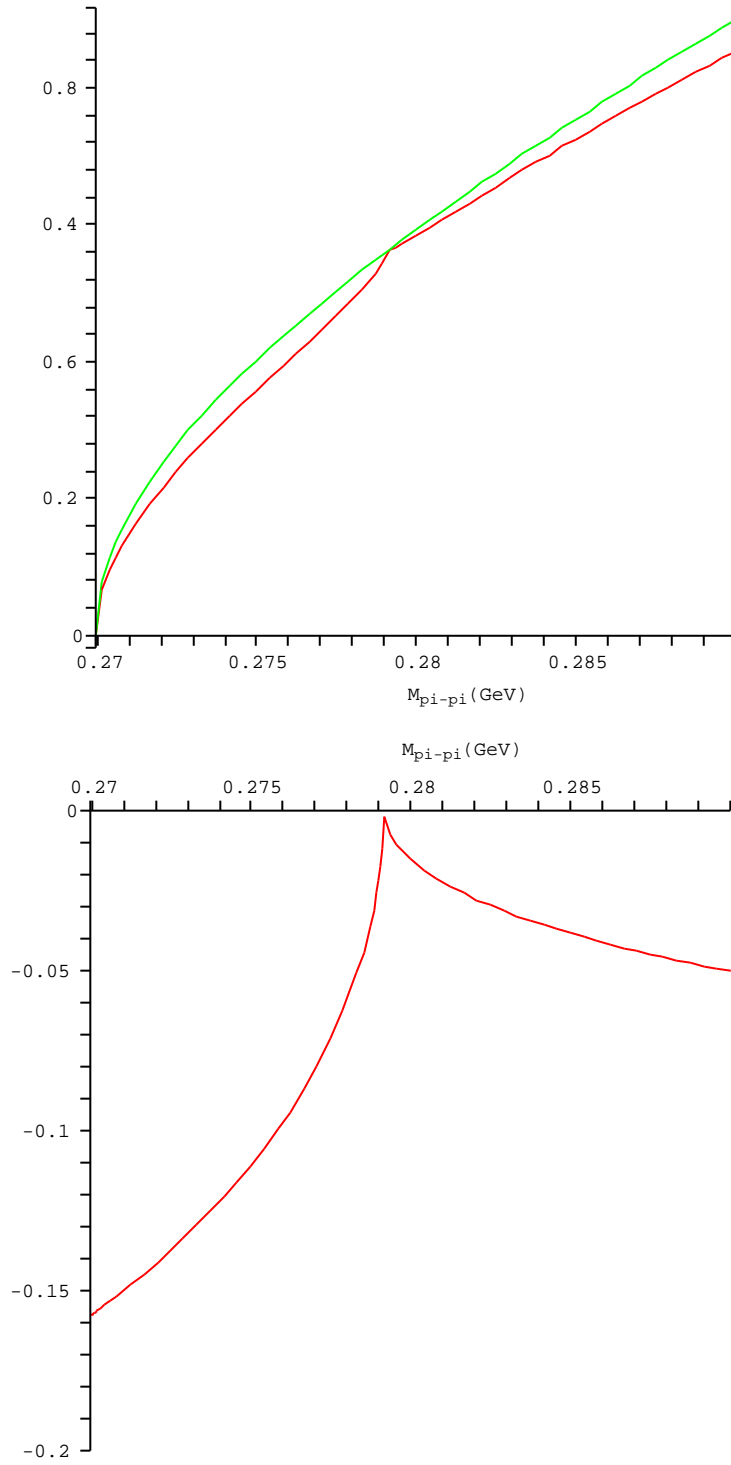
Figure 5: Illustration of the cusp effects in K^+ \rightarrow \pi^+\pi^0\pi^0 . Upper plot: differential decay distribution (in arbitrary units, as a function of the \pi^0\pi^0 invariant mass) with and without the cusp amplitude. Lower plot: relative size of the cusp amplitude with respect to the regular term. All plots have been obtained using the values of the scattering lengths and their effective ranges from Ref. [4] (see sect. 2.3).
