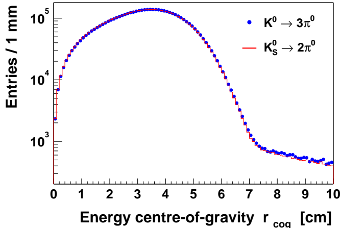
Fig. 7. Distributions of the energy centre-of-gravity r_{\text{cog}} in the LKr calorimeter for reconstructed K^0 \rightarrow 3\pi^0 (dots) and K_S \rightarrow \pi^0\pi^0 (line) near-target data events. The K_S \rightarrow \pi^0\pi^0 events have been scaled to the number of K^0 \rightarrow 3\pi^0 events.
