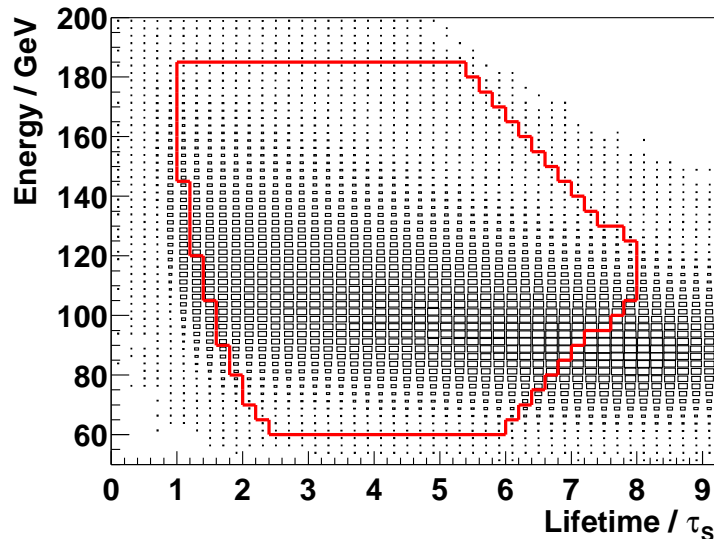
Fig. 4. Energy versus lifetime, measured from the target, of accepted K \rightarrow 3\pi^0 events from the near-target run. The contour encloses the accepted region for the \eta_{000} fit.
