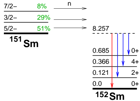
FIGURE 2. Schematic view of the neutron capture by {}^{151}\text{Sm} . The population probabilities of the first three excited target states are indicated for a temperature of kT = 30 KeV.
