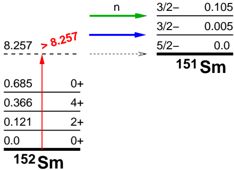
FIGURE 3. Dissociation of ^{152}\text{Sm} into ^{151}\text{Sm}+n .
