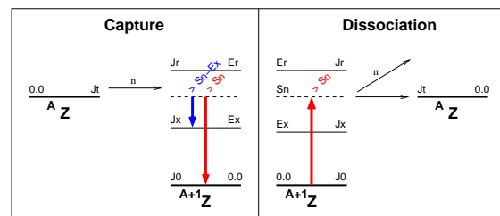
FIGURE 1. Schematic view of the neutron capture and dissociation processes
