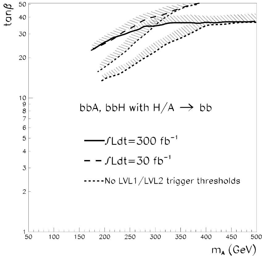
Fig. 5. In [12, Fig. 19–69]. 5\sigma -discovery contour curves for the processes bb\bar{b}H/A \rightarrow 4b , in the (m_A, \tan\beta) plane. The integrated luminosities are 30 \text{ fb}^{-1} (dashed line) and 300 \text{ fb}^{-1} (solid line). The dotted lines show the expected extension in coverage if the level-1 and level-2 trigger thresholds are not applied.
