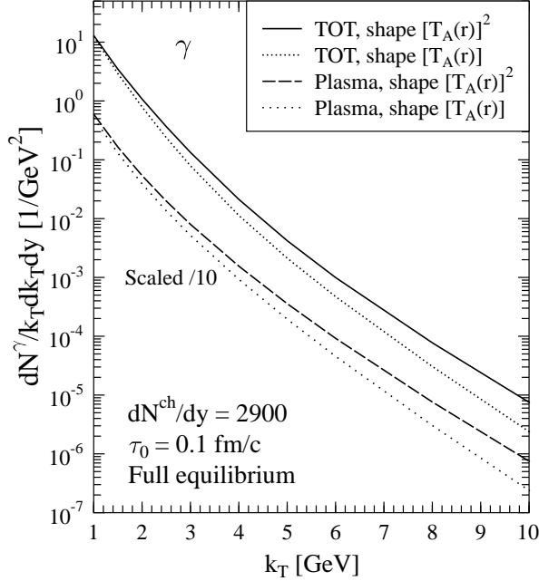
Fig. 61: Photon spectra when the shape of initial condition is taken to be [T_A(r)]^\alpha with \alpha = 1 or 2 . dN_{ch}/dy \simeq 2900 and \tau_0 = 0.1 fm/c in both cases.
