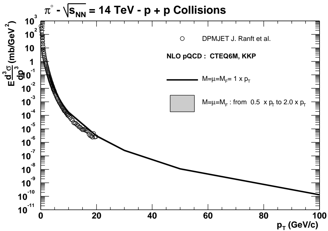
Fig. 29: Same as Fig. 28 but at \sqrt{s} = 14 \text{ TeV} .
