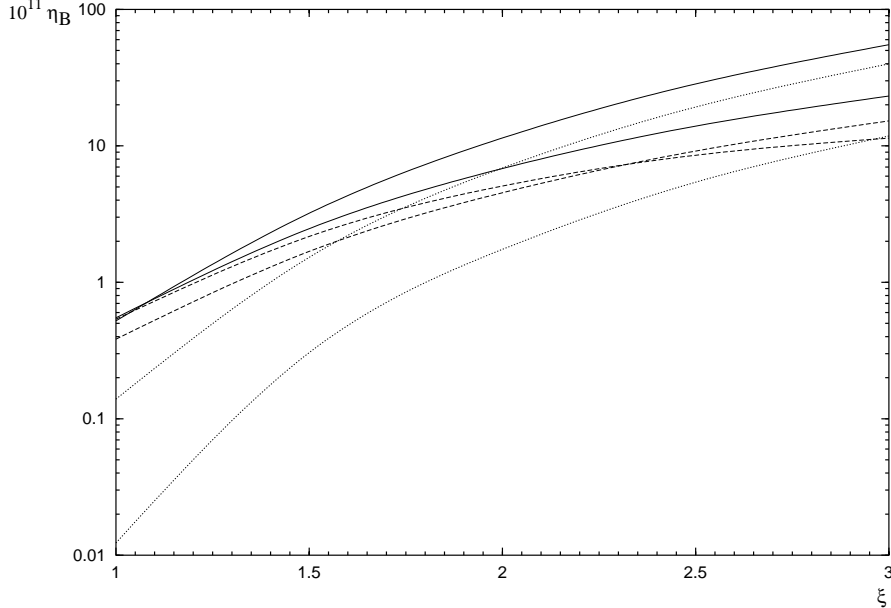
Figure 5: The baryon asymmetry as a function of \xi for two wall velocities. The different line types have the same meaning as in fig. 4, and again L_w = 8/T and M = 6T . On the right edge of the figure the upper curves are for v_w = 0.01 and the lower ones for v_w = 0.3 .
