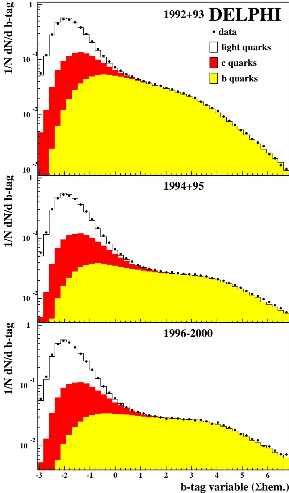
Figure 1: Comparison between data and simulation of the normalised number of events versus the b -tag variable for 1992+93 (upper plot), 1994+95 (middle) and 1996-2000 (lower plot). The b -, c - and light quark composition of the simulation has been reweighted according to the measured branching fractions [12]. The b - and c -quark simulation correction from Section 4.3 is not applied at this stage.
