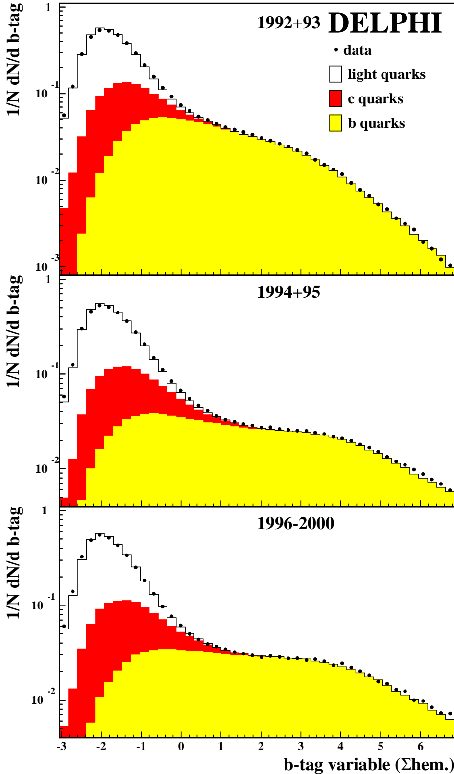
Figure 1: Comparison between data and simulation of the normalised number of events versus the b\text{-tag variable} for 1992+93 (upper plot), 1994+95 (middle) and 1996-2000 (lower plot). The b -, c - and light quark composition of the simulation has been reweighted according to the measured branching fractions [12]. The b - and c -quark simulation correction from Section 4.3 is not applied at this stage.
