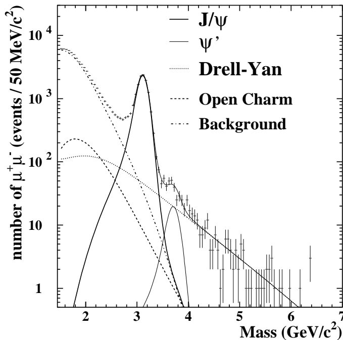
Figure 3: Opposite-sign dimuon invariant mass spectrum for the centrality class 35 < E_T < 45 GeV. The results from the fit are also shown.
