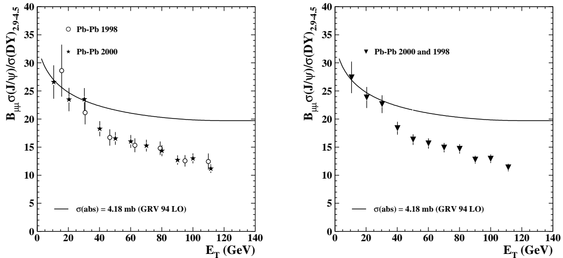
Figure 10: Comparison between 1998 and 2000 results: separate (J/\psi)/ Drell-Yan cross-sections ratios from 1998 and 2000 (left) and weighted average (right), as a function of transverse energy.
