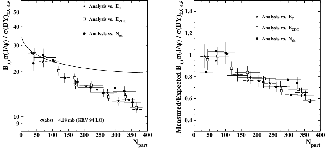
Figure 7: The (J/\psi) / \text{Drell-Yan} cross-sections ratio as a function of N_{\text{part}} for three analyses of the Pb-Pb 2000 data sample, compared to (left) and divided by (right) the normal nuclear absorption pattern.
