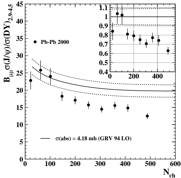
Figure 6: The (J/\psi) / Drell-Yan cross-sections ratio as a function of charged multiplicity for the Pb-Pb 2000 data sample. The inset shows the ratio Measured/Expected, i.e. data over normal nuclear absorption.
