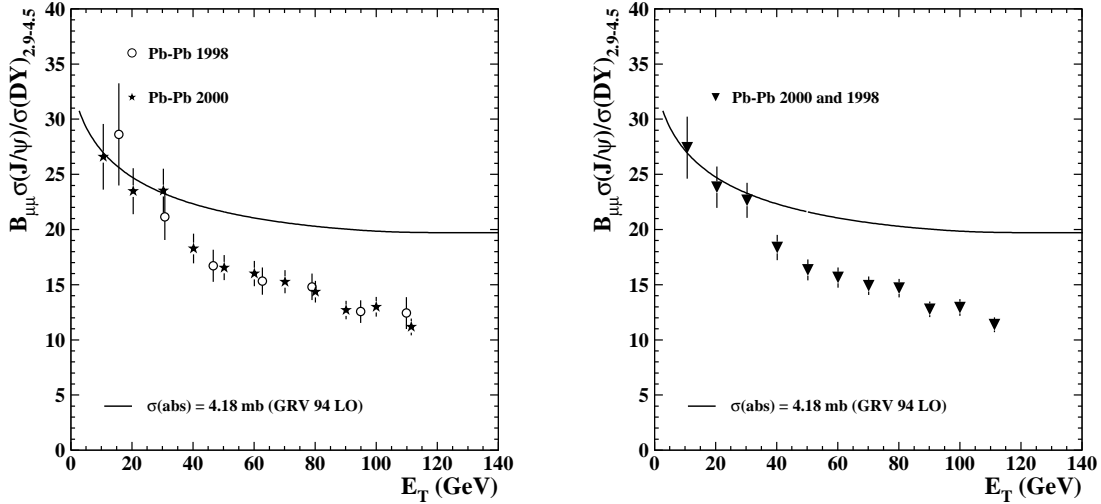
Figure 10: Comparison between 1998 and 2000 results: separate (J/\psi) / \text{Drell-Yan} cross-sections ratios from 1998 and 2000 (left) and weighted average (right), as a function of transverse energy.
