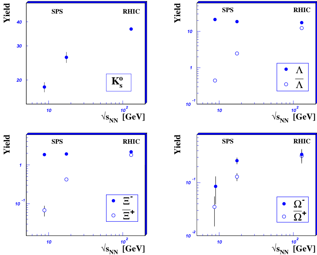
Figure 1. K_S^0 and hyperon yields at central rapidity in nucleus-nucleus collisions at SPS and RHIC energies. Large error bars on the \Xi and \Omega yields are due to the restriction of the NA57 data sample to the STAR centrality ranges.
