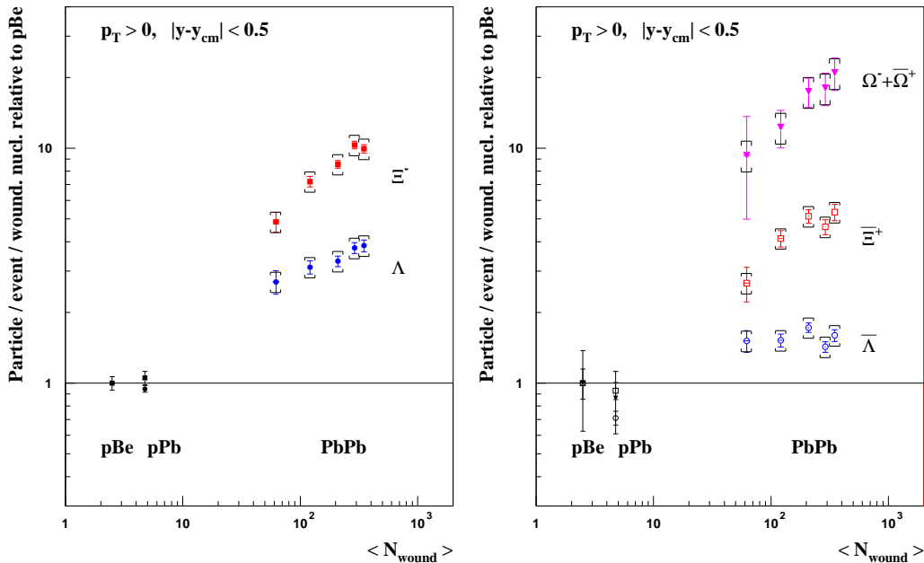
Figure 4. Centrality dependence of hyperon enhancements at 158 A GeV/c. The error bars indicate the statistical errors only, while the bracket symbols represent the systematic errors.
