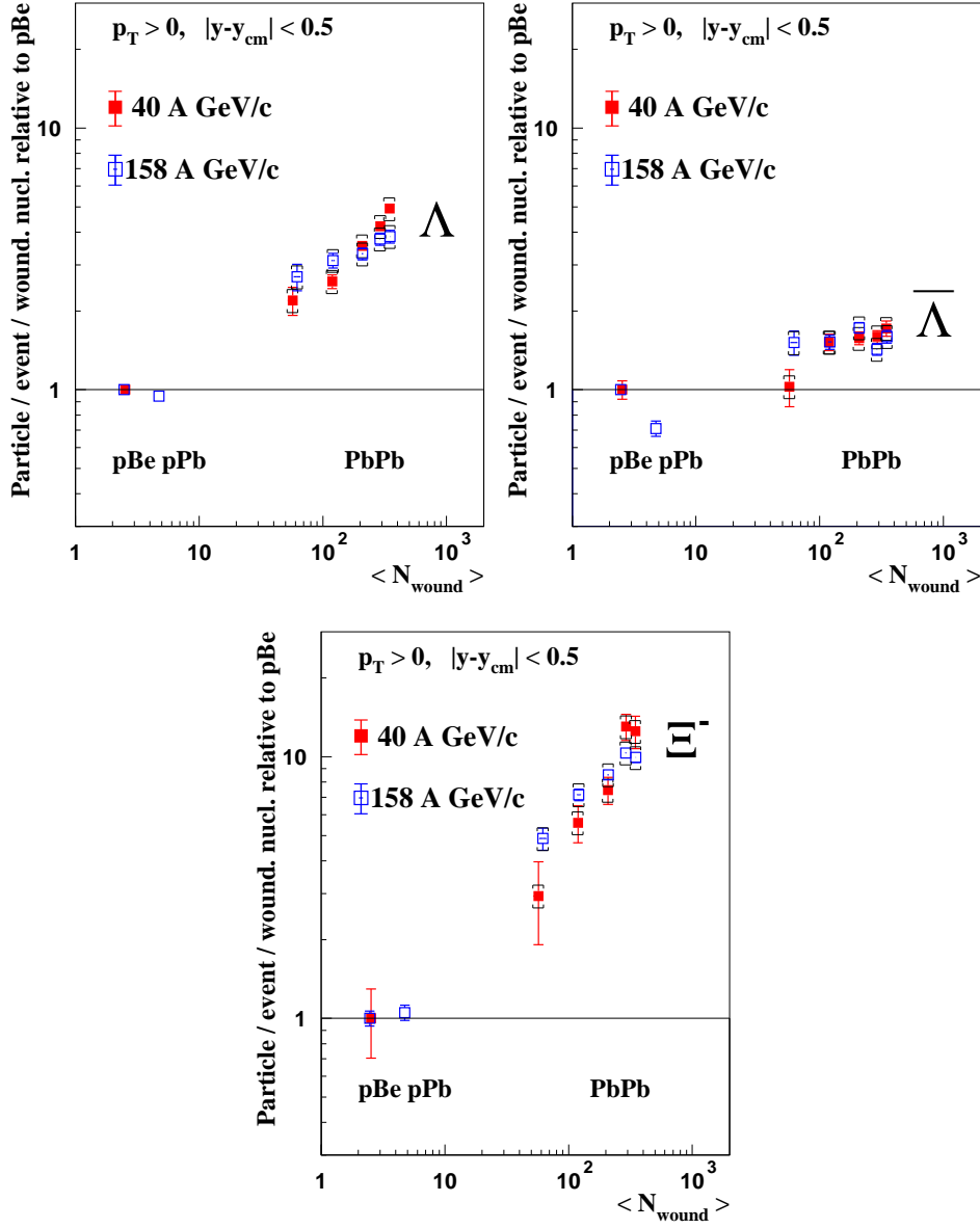
Figure 5. Centrality dependence of \Lambda , \bar{\Lambda} and \Xi^- enhancements at both 158 and 40 A GeV/c. The error bars indicate the statistical errors only, while the bracket symbols represent the systematic errors.
