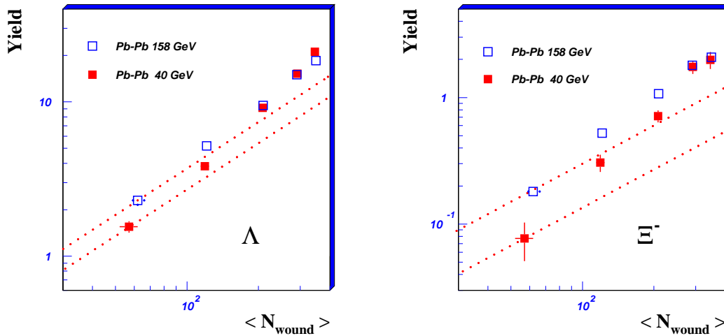
Figure 3. Centrality dependence of \Lambda and \Xi^- yields in Pb-Pb collisions at SPS.
