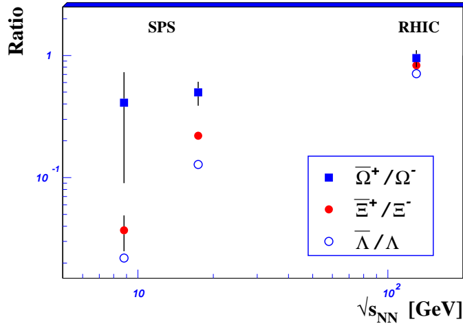
Figure 2. Antihyperon to hyperon ratios in nucleus-nucleus collisions at SPS and RHIC.
