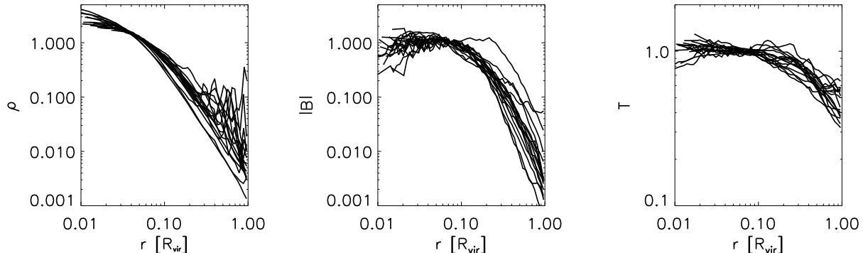
Fig. 2.— Spherically averaged profiles of gas density (left panel), magnetic field strength (middle panel) and temperature (right panel, mass-weighted) for the 16 most massive clusters extracted from the simulation. The profiles are scaled to R_{\text{vir}} and normalized to have the same mean value within 0.1 \times R_{\text{vir}} .
