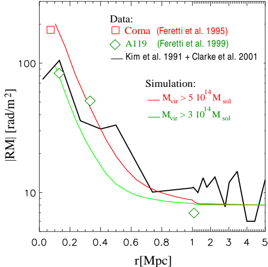
Fig. 4.— Comparison of RMs from the simulation with observations for Abell clusters, as a function of distance to the closest cluster. Smooth lines represent median values of |RM| produced by simulated clusters with masses above 5 \times 10^{14} M_{\odot} and 3 \times 10^{14} M_{\odot} . The broken line represents the median of combined data taken from the independent samples in Kim et al. (1991) and Clarke et al. (2001). We also include data (diamonds) for the three elongated sources observed in A119 (Feretti et al. 1999a), and for the elongated source observed in the Coma cluster (Feretti et al. 1995).
