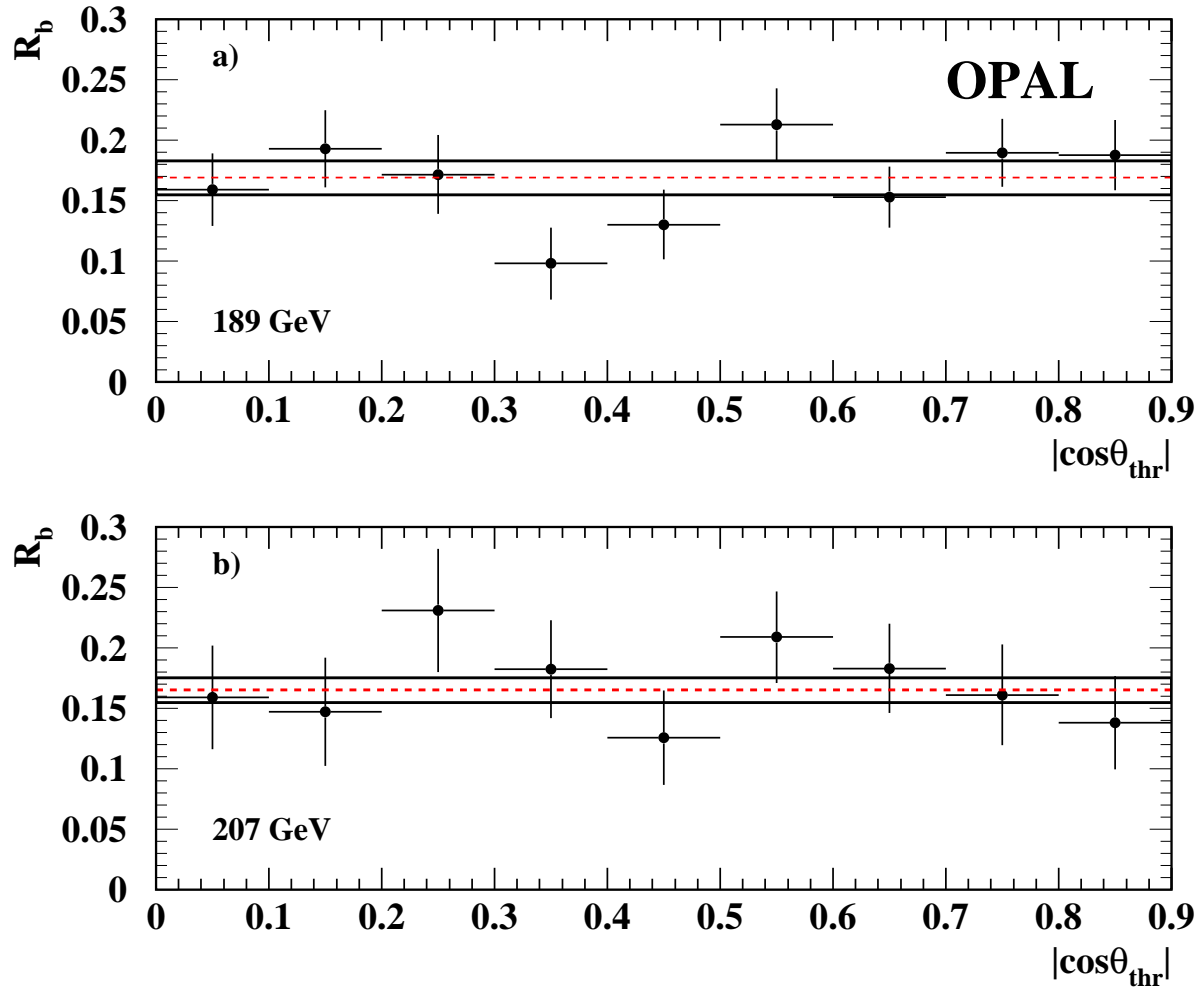
Figure 2: Measured values of R_b for: a) the 189 GeV sample; b) the 207 GeV sample with statistical uncertainties only. The dashed line is the average value and the solid lines show the the band corresponding to the one standard deviation uncertainty.
