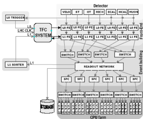
Figure 2: LHCb online dataflow
