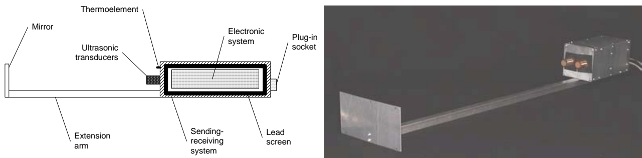
Figure 3. Schematic and general view of the sound-velocity measuring unit
