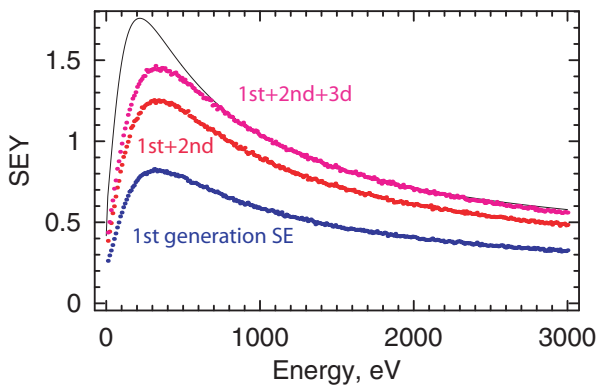
Figure 7: Secondary emission yield in magnetic field, \alpha = 40^\circ .
