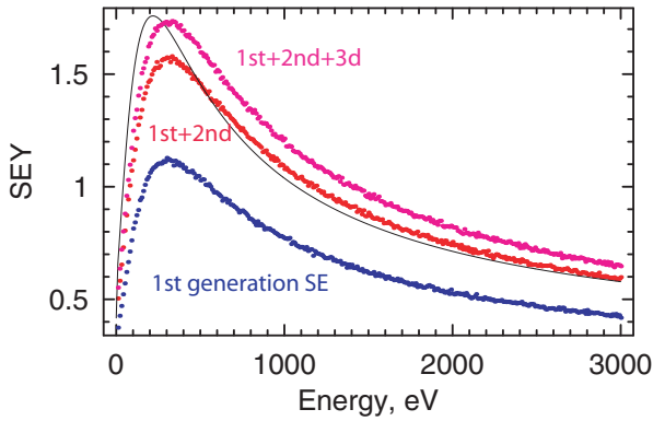
Figure 6: Secondary emission yield in a magnetic field, \alpha = 60^\circ .
