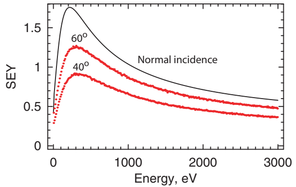
Figure 4: Comparison of the effective SEY for 60^\circ and 40^\circ grooves.
