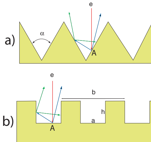
Figure 1: Triangular (a) and rectangular (b) grooves on the surface. Triangular grooves are characterized by the angle \alpha . Rectangular grooves have a period b , width a and depth h .
