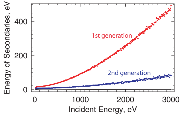
Figure 3: Energy of secondary electrons for triangular grooves with an angle \alpha = 60^\circ .
