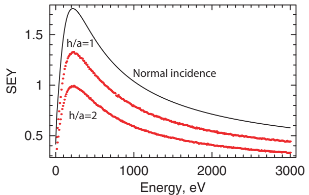
Figure 5: Rectangular grooves.
