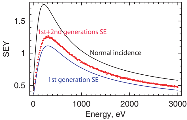
Figure 2: SEY as a function of incident energy for triangular grooves with \alpha = 60^\circ .
