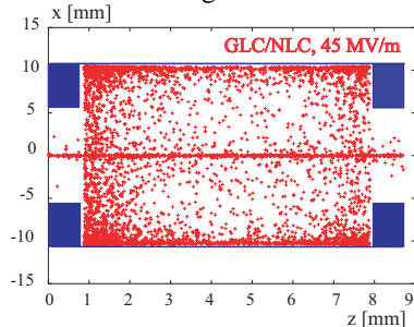
Figure 6: Snapshot of electron z - x distribution after the last bunch passage for GLC/NLC at nominal rf gradient.
