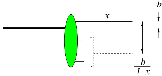
Figure 1: A three-quark configuration in the mixed representation of definite transverse position and definite plus-momentum. x denotes the plus-momentum fraction of the upper quark with respect to the nucleon. The dashed line indicates the center of momentum of the two lower quarks and the thick solid line the center of momentum of the proton.
