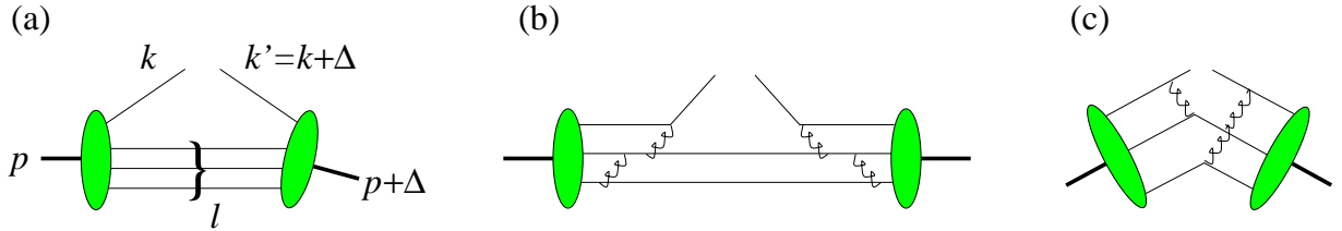
Figure 12: (a) Momenta of nucleon, active quark and spectator system in a GPD. (b) Perturbative mechanism for large x . (c) Hard-scattering mechanism [47] for large t .
