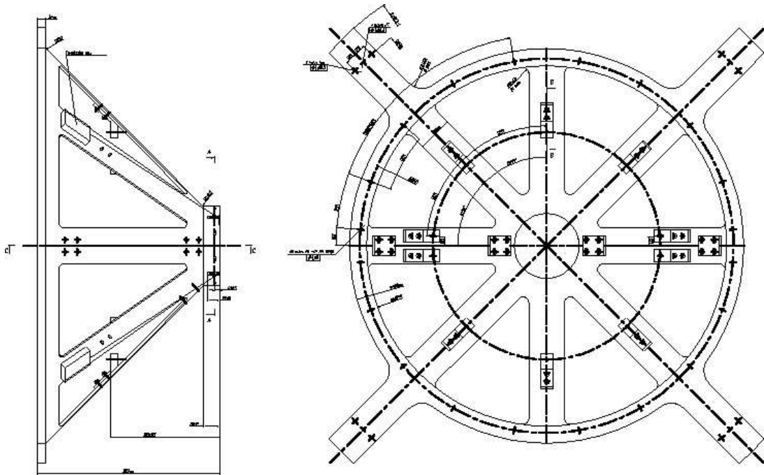
Figure 4.37: Preliminary technical drawing of the FMD3 cone
