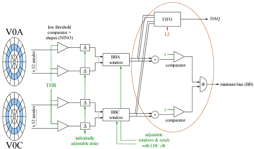
Figure 3.23: Minimum-bias trigger.
