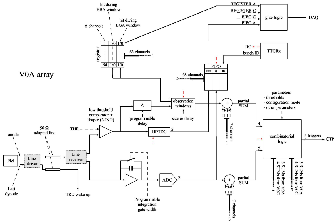
Figure 3.20: V0 Front-End Electronics scheme.
