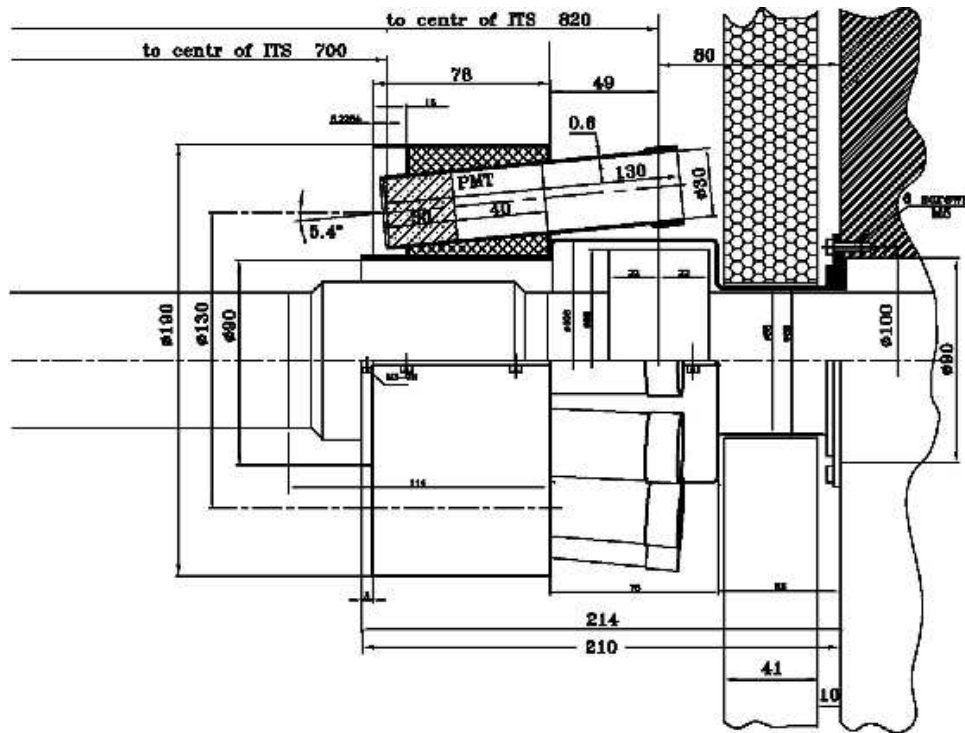
Figure 2.12: Layout of the T0 support on the muon absorber side.
