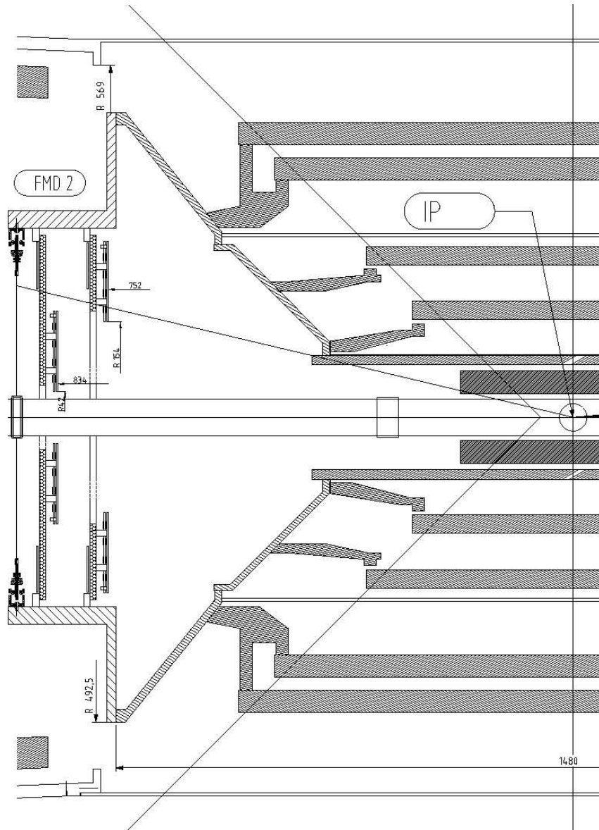
Figure 4.4: Cross section of FMD2 on the RB24 side of the IP. The two FMD2 rings are shown at z = 752 mm and z = 834 mm from the IP and attached to their cylindrical mechanical support. This support also supports the beam pipe.
