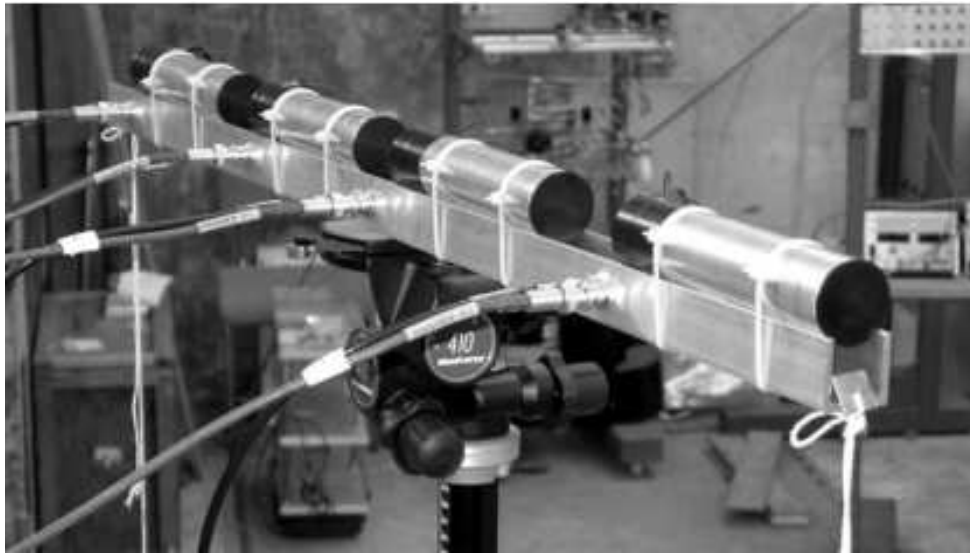
Figure 2.42: Photograph of a typical detector configuration during the 2004 test run at CERN PS. There are four PMT + quartz detector units. Each unit has its own aluminum casting with plastic end cups.
