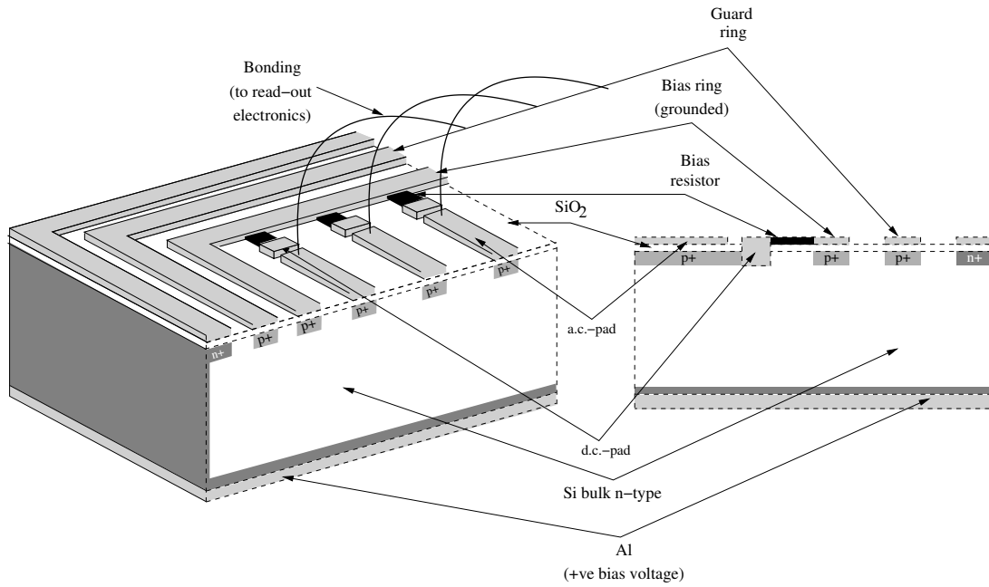
Figure 4.21: Left: a three-dimensional schematic view of the corner of a silicon sensor, showing the placement of guard ring, voltage distribution, etc. Right: a two-dimensional cross-section through the silicon wafer parallel to the direction of the active strips.
