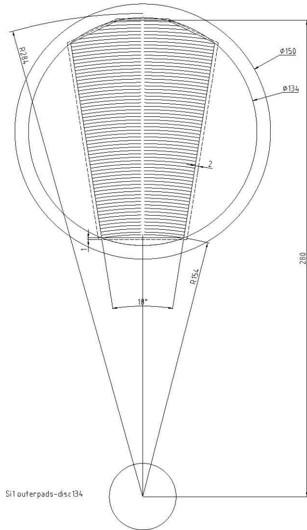
Figure 4.23: Geometry of an outer silicon strip sensor manufactured from a 6 inch Si wafer. The active parts of the detector must stay within the circle of diameter 134 mm for manufacturing reasons. The active area of the wedge-shaped sensor is outlined with full drawn lines, while the slightly larger area indicated with the dashed line represents the physical size of the cut wafer, including bias and guard ring structures. Each sector is subdivided into two azimuthal sectors, each with 256 strips at constant pitch (a smaller number is shown for clarity).
