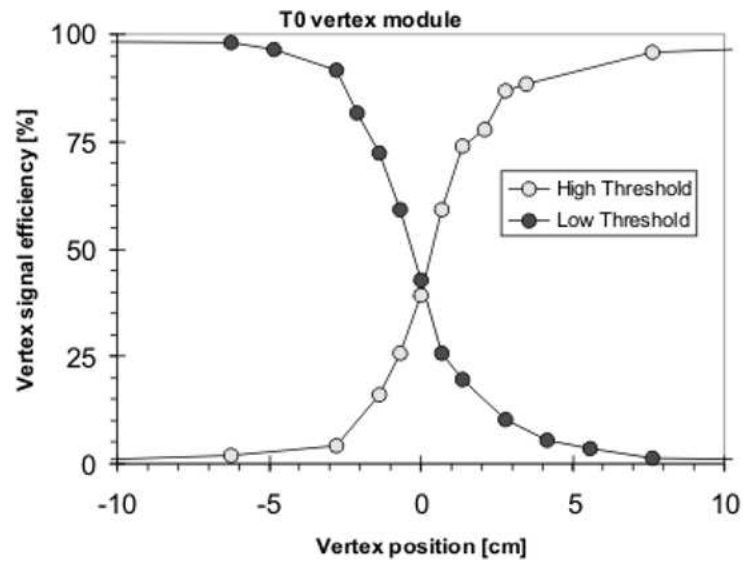
Figure 2.36: Performance of the first prototype T0 Vertex Unit during the July 2003 test experiment using PS beams at CERN.
