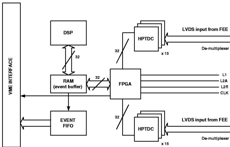
Figure 2.54: TRM unit.
