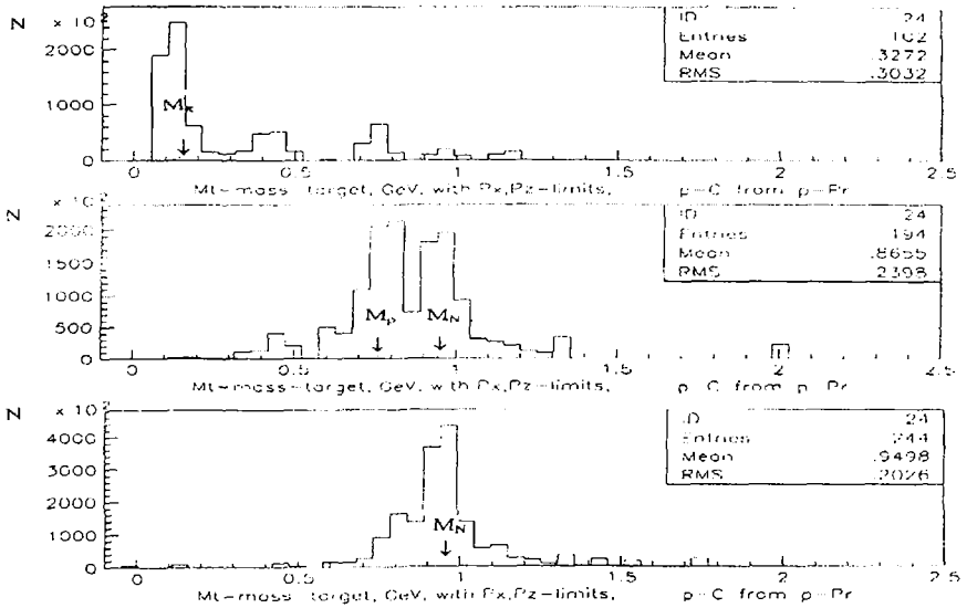
Fig. 4B. Mass-target M_1 distributions of the candidates for separate reactions of protons with (from top to bottom correspondingly), \pi^- mesons, \pi^+ mesons and nucleons for pC interactions.
