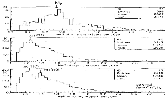
Fig. 7. Effective mass distributions for pp-quasi-interactions shifted on from C+C, 11, interactions. Method MPMR for background restriction at n=3 was applied here: (Top) - the effective mass distributions of \pi^+\pi^- pions - M_{\rho} ; (Middle) - M_{\Delta} ; (Bottom) - M_{N} .
