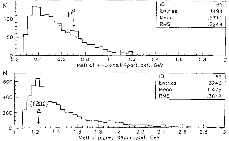
Fig. 9. Two particle effective mass distributions (top) M_{\pi^+\pi^-} and (bottom) M_{p\pi^+} , obtained by method MPMR at n=4 for CC-interactions.
