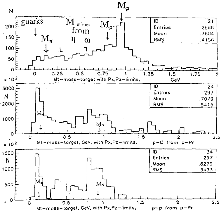
Fig. 3 Mass-target ( M_t ) distributions with transverse momentum balance: \Delta \Sigma p_t = \text{sqrt}((\Sigma p_{tx})^2 + (\Sigma p_{ty})^2) = \pm 140 \text{ Mev}/c . (Top): C-C-interactions without weights, (Middle) p-C-interactions from p-C 3 H 8 -interactions with the weights 'wt', 'wp' and 'we'; (Bottom) p-p-interactions from p-C 3 H 8 -interactions with the weights 'wt', 'wp' and 'we'.
