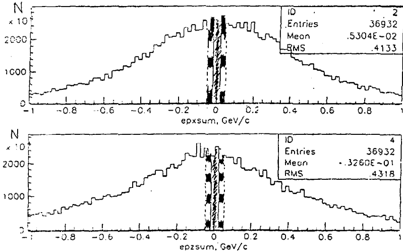
Fig 2. Summary transverse momentum components \Sigma p_{xi} and \Sigma p_{zi} for all measured CC-interactions. The request of the transverse momentum compensation means that the \Sigma p_{xi} and \Sigma p_{zi} do not exceed any small value simultaneously – only the events from the narrow stripes of \Sigma p_{xi} and \Sigma p_{zi} are taken for the analysis.
