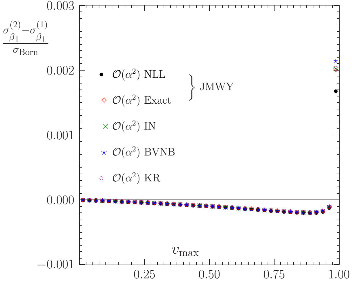
Figure 3: Difference \bar{\beta}_1^{(2)} - \bar{\beta}_1^{(1)} for the YFS3ff MC (the EEX3 option in the \mathcal{K}\mathcal{K} MC), as a function of the cut v_{\max} . It is divided by the Born cross-section. The comparisons are the same as in Fig. 2.
