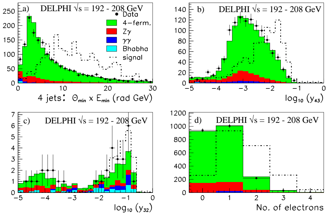
Figure 4: LL \bar{E} : sparticle pair search in multi-lepton channels – Distributions of variables used in the four analyses, as described in the text: a) gaugino, b) slepton, c) sneutrino tau, d) squark. The simulated signals correspond to production of a) \tilde{\chi}_2^0 \tilde{\chi}_1^0 and \tilde{\chi}_1^+ \tilde{\chi}_1^- ( m_{\tilde{\chi}_1^0} = 50 \text{ GeV}/c^2 , m_{\tilde{\chi}_2^0} = 85 \text{ GeV}/c^2 , m_{\tilde{\chi}_1^\pm} = 95 \text{ GeV}/c^2 ), b) \tilde{\nu}_e \tilde{\nu}_e ( m_{\tilde{\nu}_e} = 100 \text{ GeV}/c^2 ), c) \tilde{\nu}_\tau \tilde{\nu}_\tau ( m_{\tilde{\nu}_\tau} = 95 \text{ GeV}/c^2 ), d) \tilde{t}\tilde{t} ( m_{\tilde{t}} = 95 \text{ GeV}/c^2 ) (the signal normalisation is arbitrary).
