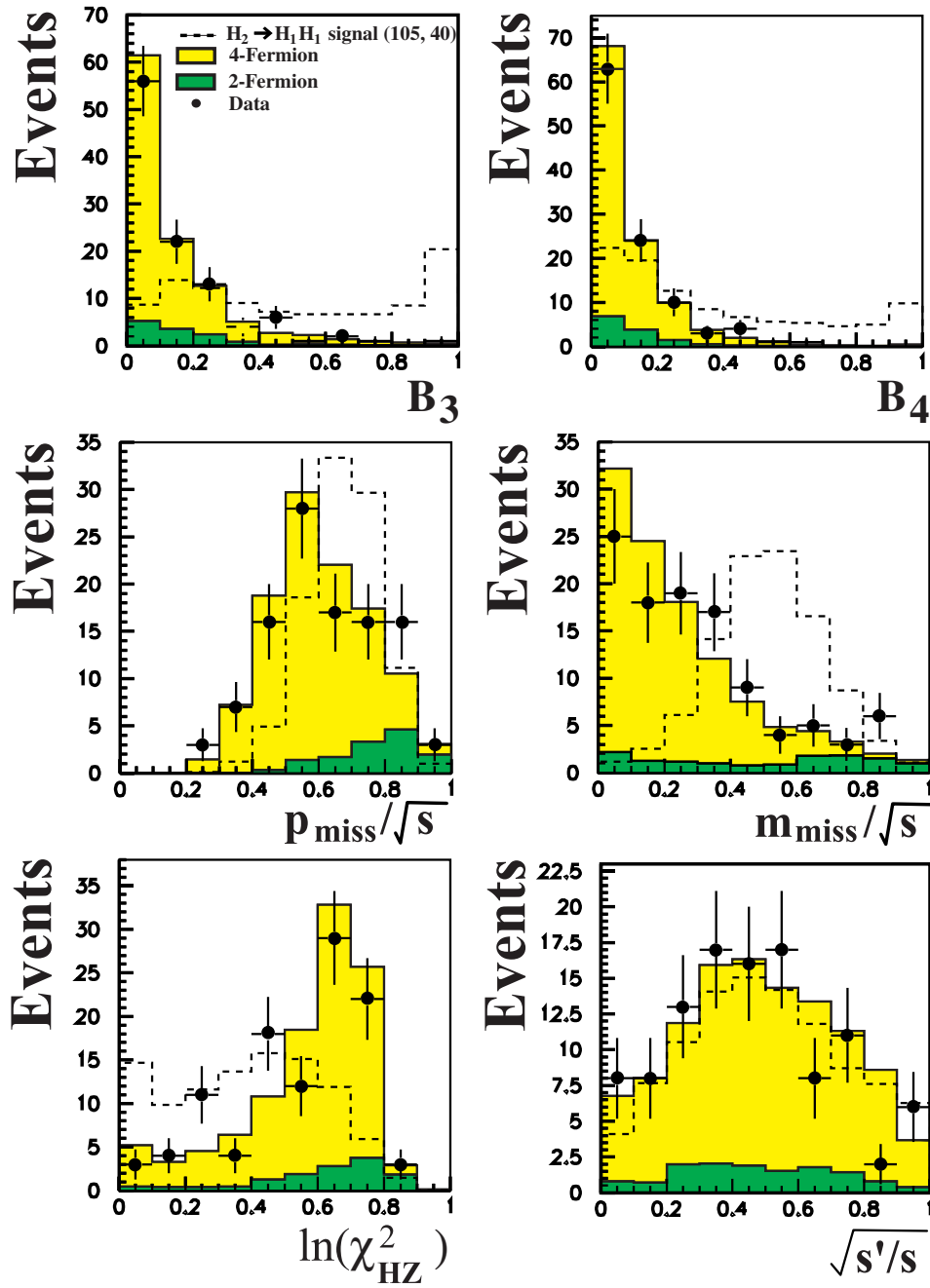
Figure 2: Distributions of some ANN input variables for subsample B for e^+e^- \rightarrow \mathcal{H}_2 Z \rightarrow b\bar{b}\nu\bar{\nu} and e^+e^- \rightarrow \mathcal{H}_1 \mathcal{H}_1 Z \rightarrow b\bar{b}b\bar{b}\nu\bar{\nu} (see Section 4.1.2) in the region 100 \text{ GeV} < m_{\mathcal{H}_2} < 110 \text{ GeV} .
